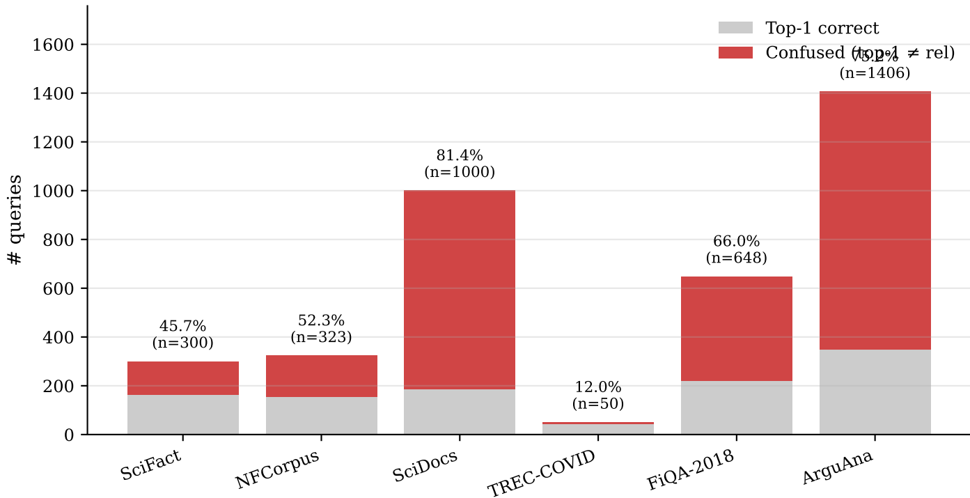
Confused-slice base rate per dataset (top-1 \neq relevant)
