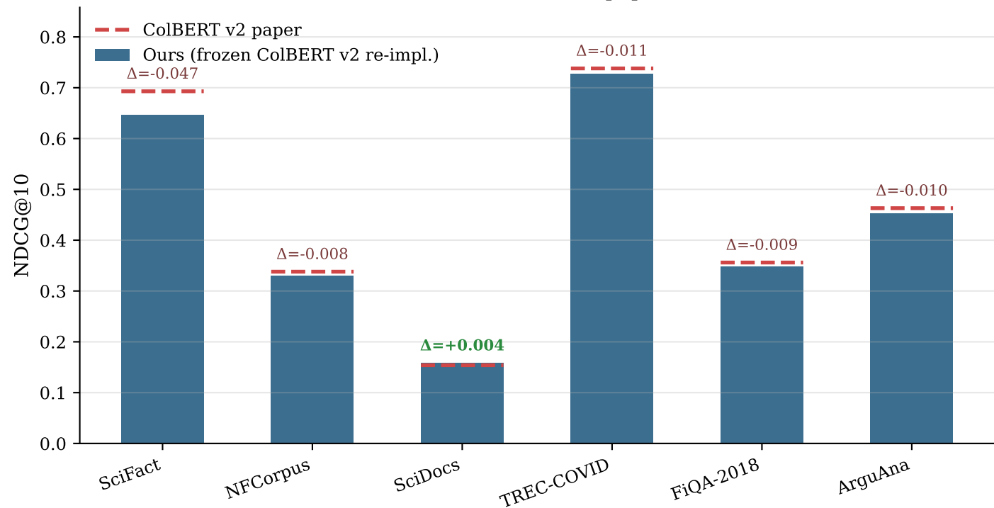
Baseline NDCG@10 vs ColBERT v2 paper (zero-shot BEIR)
