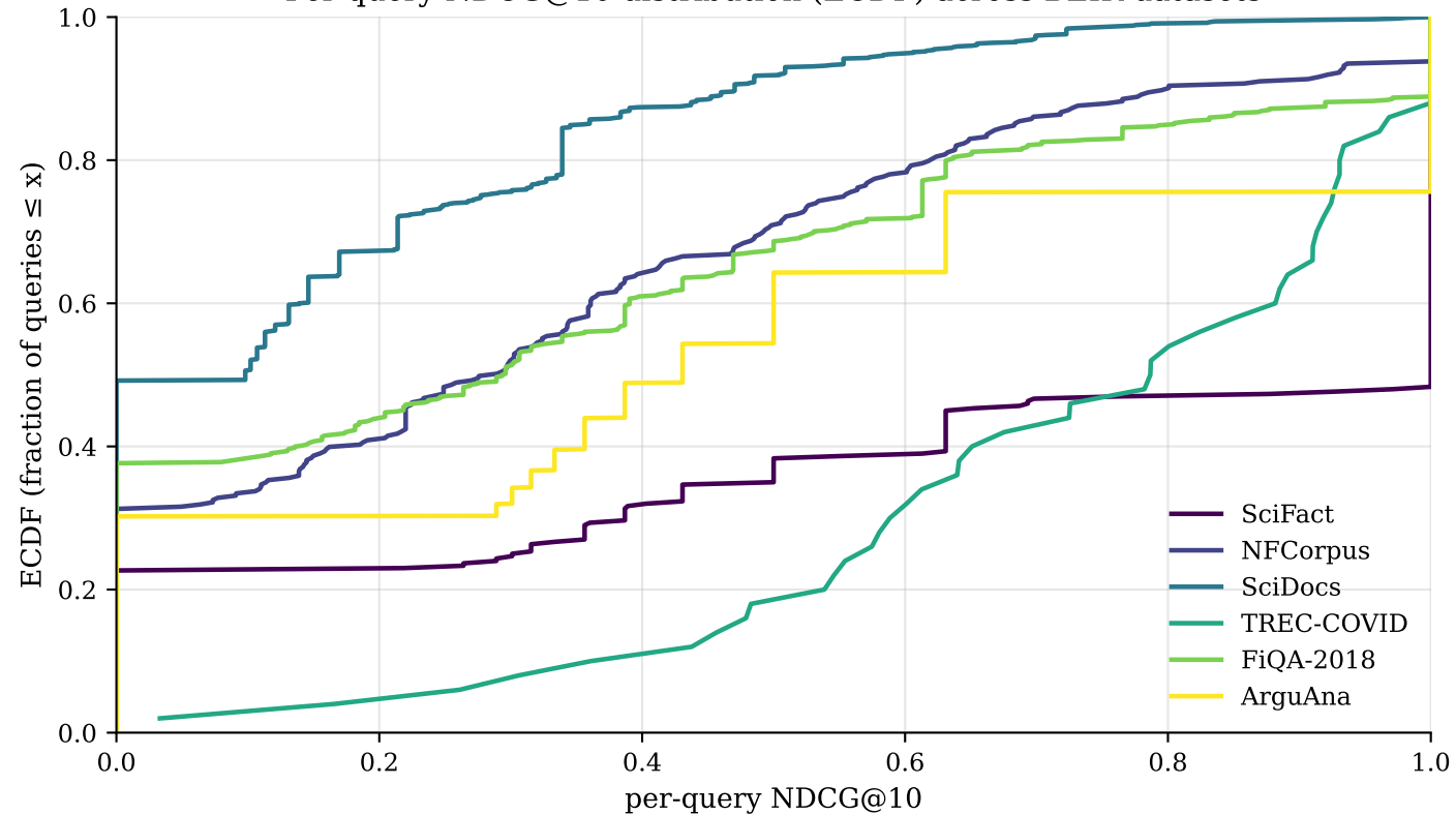
Per-query NDCG@10 distribution (ECDF) across BEIR datasets
