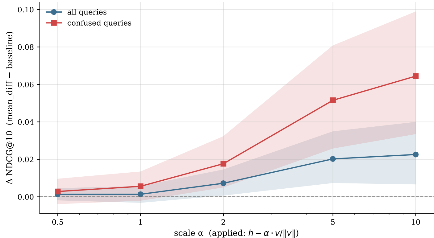
Magnitude sweep on SciFact: 95 % paired bootstrap CI vs \alpha
