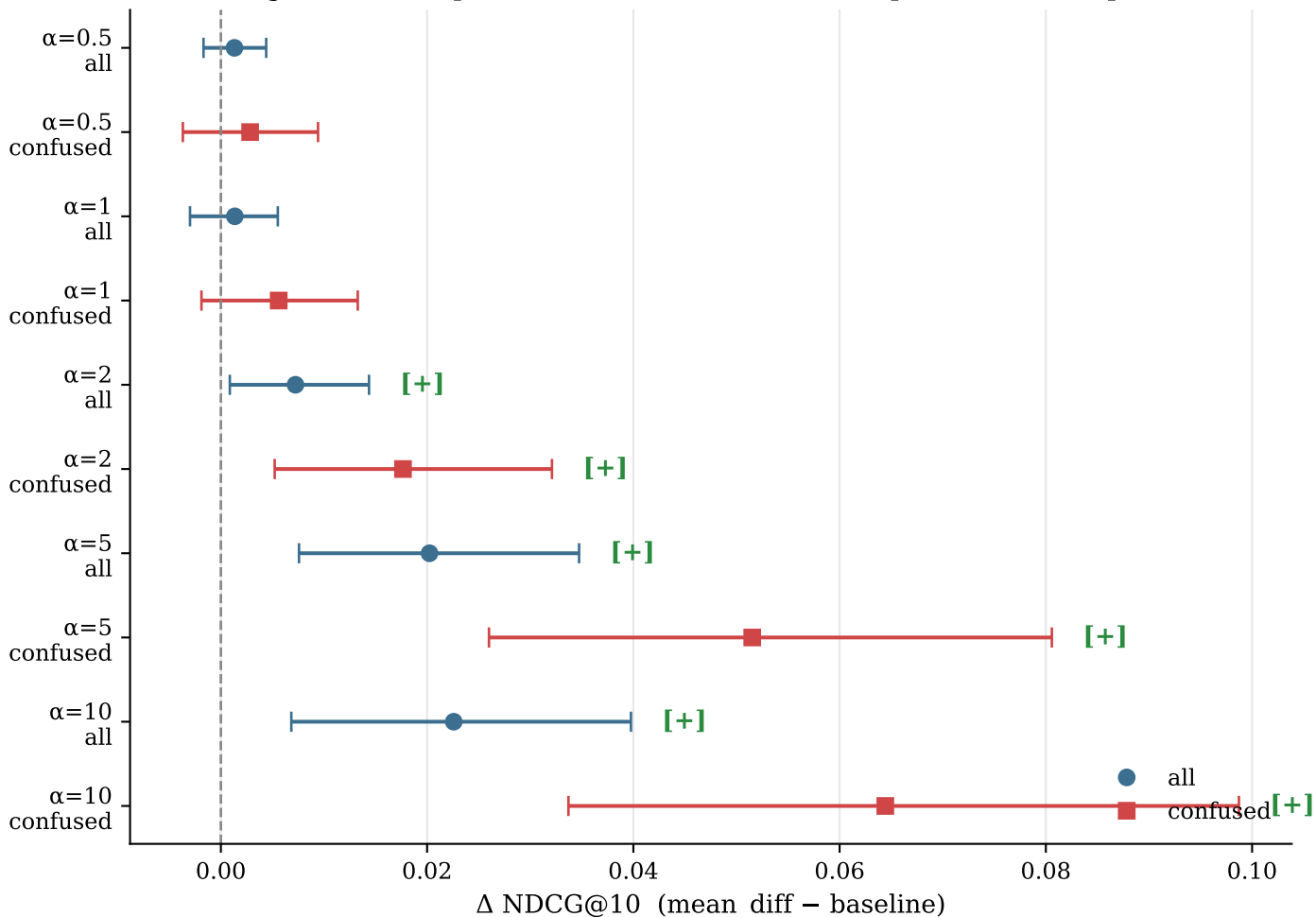
Magnitude sweep on SciFact: forest CIs (95 %, paired bootstrap 10K)
