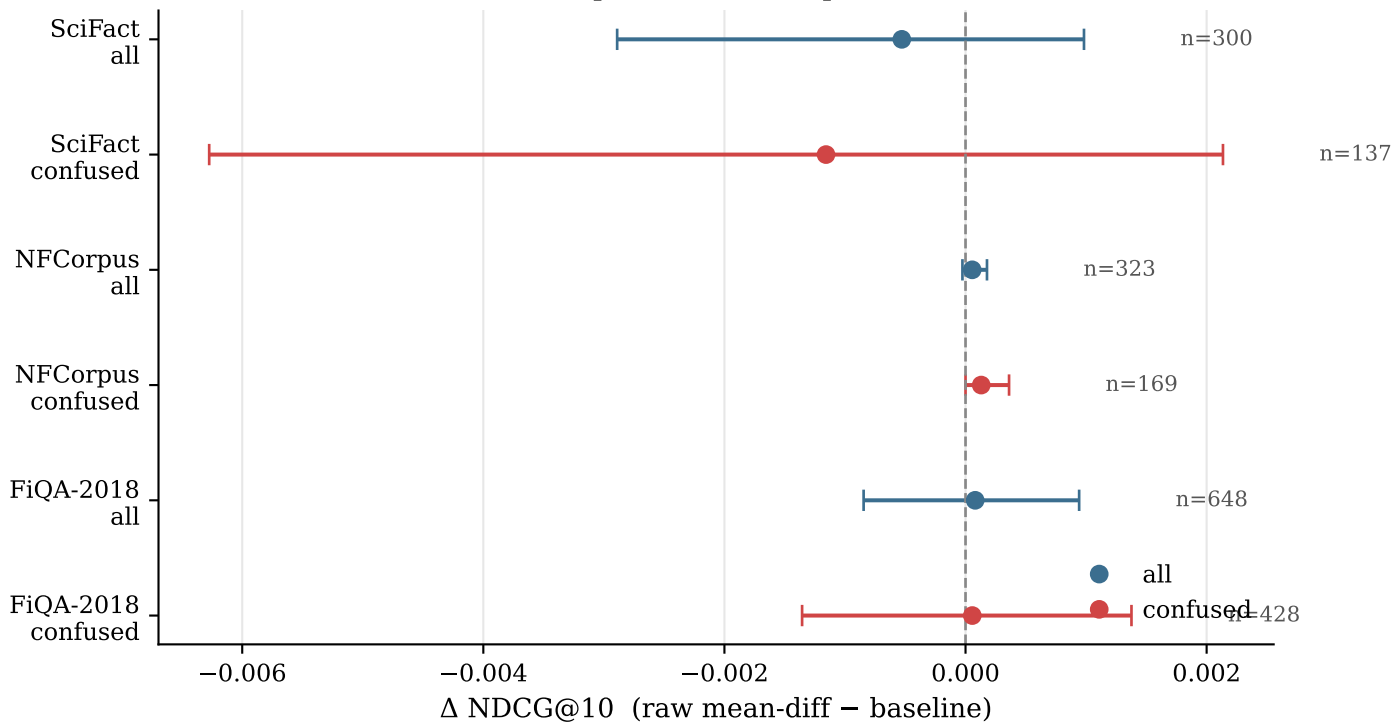
Raw unscaled mean-diff: paired bootstrap 95 % CI on \Delta NDCG@10
