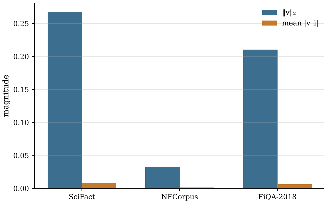
Magnitude of raw mean-diff direction \mathbf{v} per dataset
