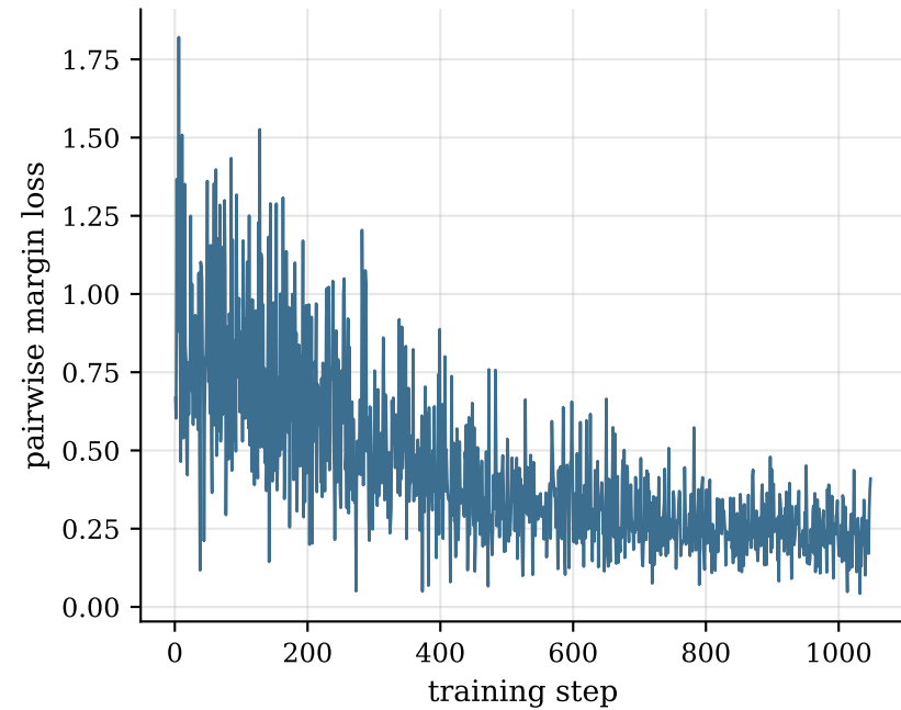
Train loss (rank)
