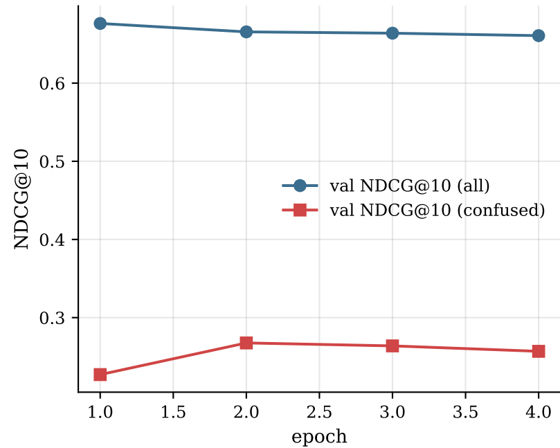
Validation curves (early-stop signal)
