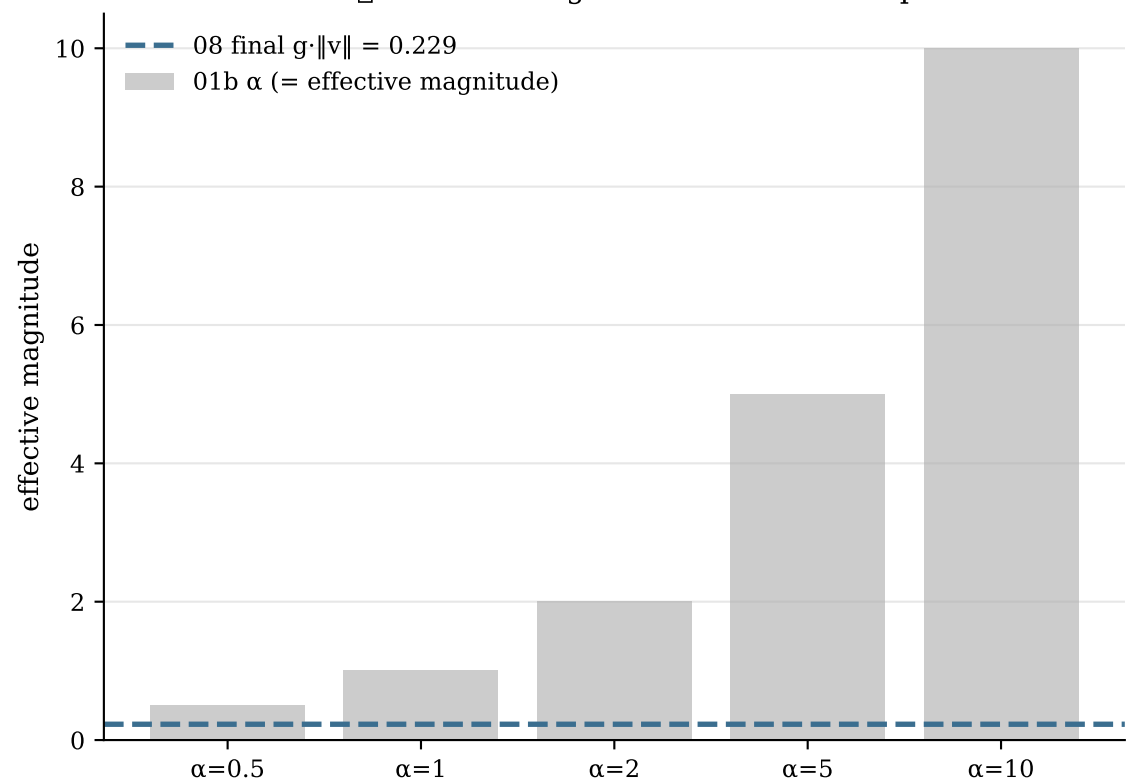
08 \square effective magnitude vs 01b \alpha sweep
