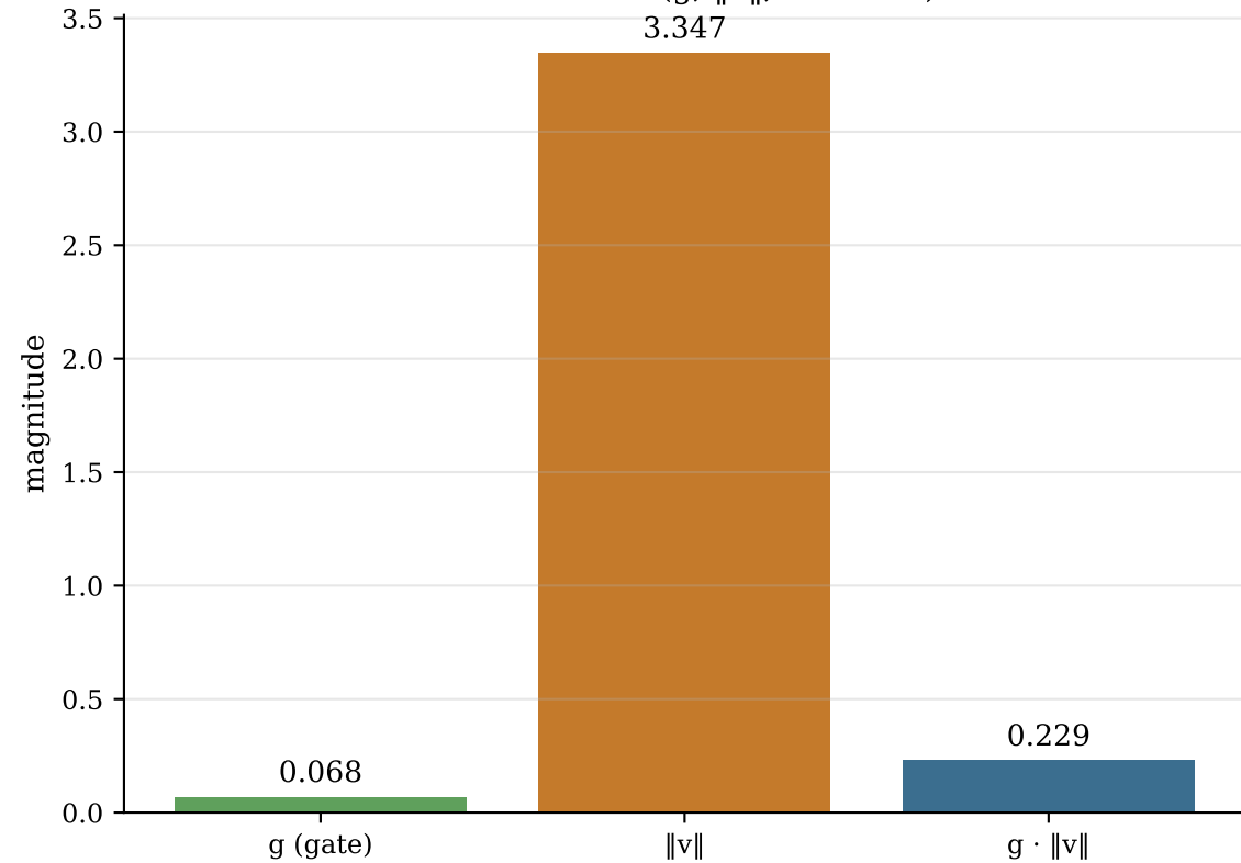
Final learned (g, \|v\| , effective)
