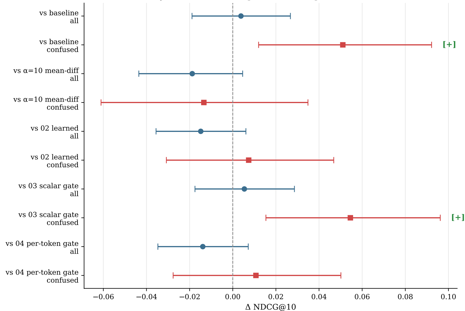
05 (5-layer learned LSR) — paired bootstrap 95 % CI vs 5 anchors
