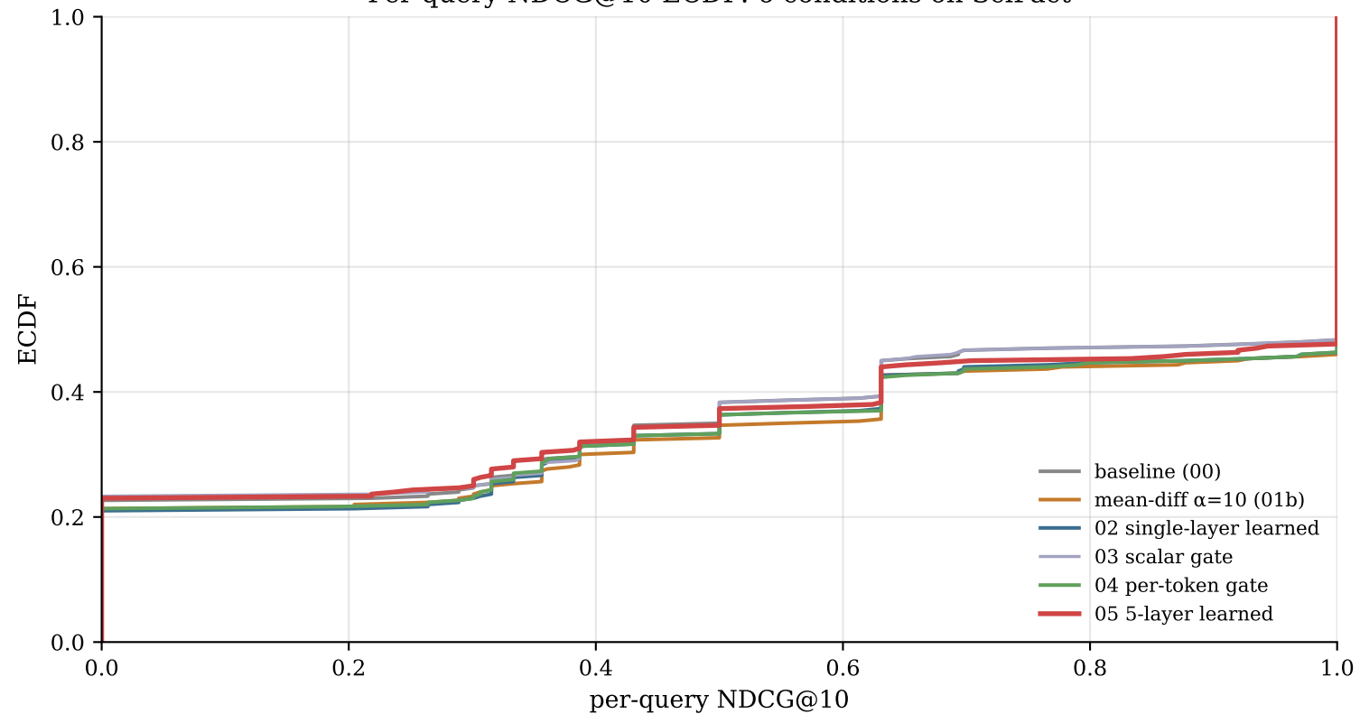
Per-query NDCG@10 ECDF: 6 conditions on SciFact
