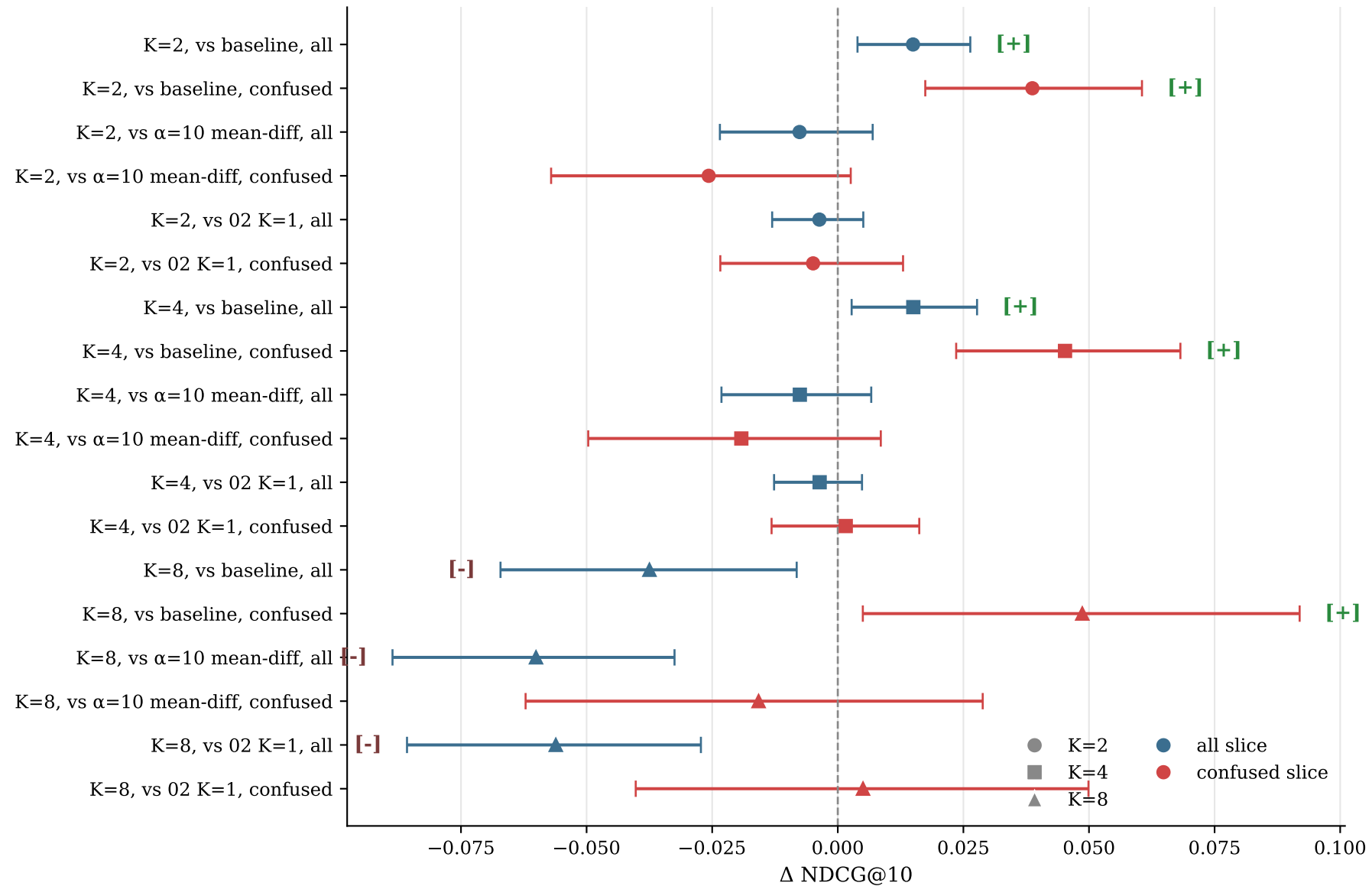
K-sweep: paired bootstrap 95% CI on \Delta NDCG@10
