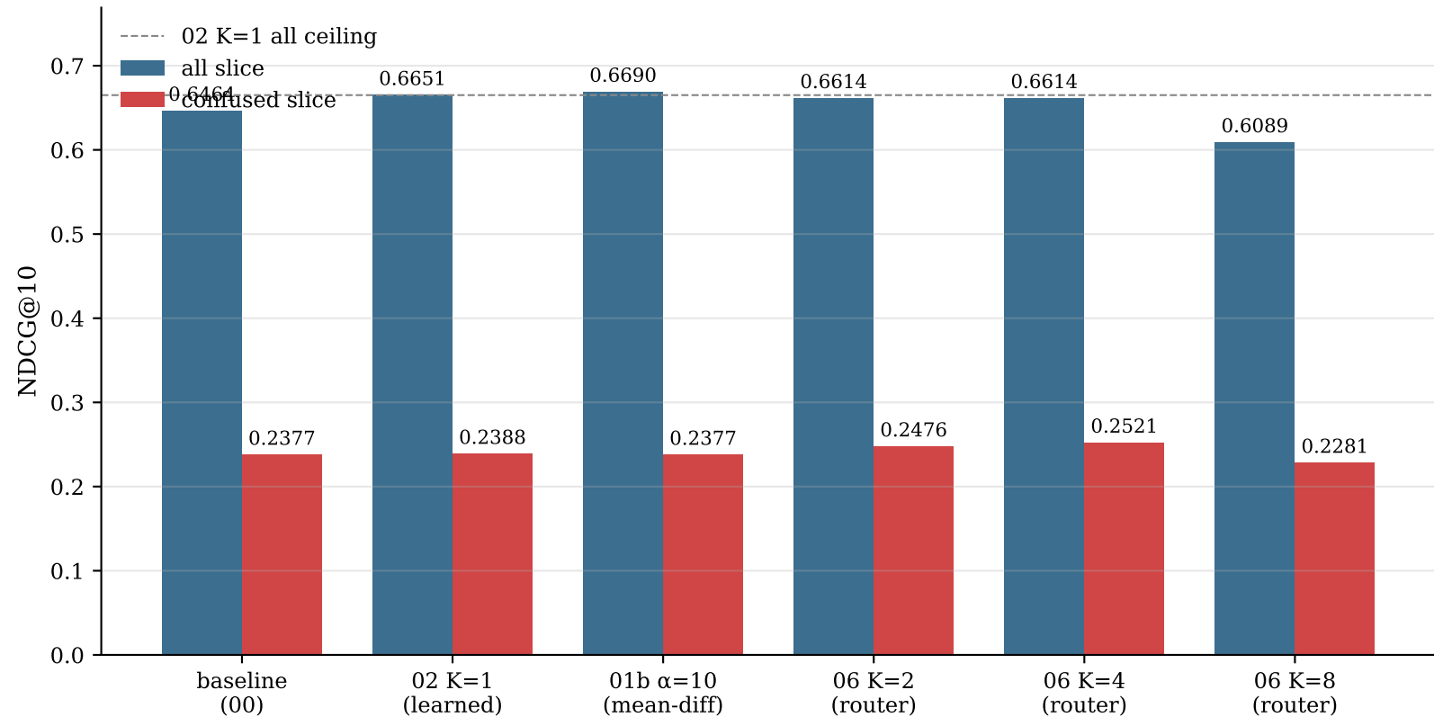
K sweep: NDCG@10 across K (translation-family ceiling test)
