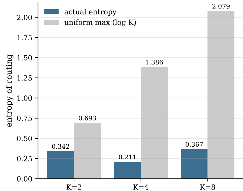
Routing entropy vs uniform max
