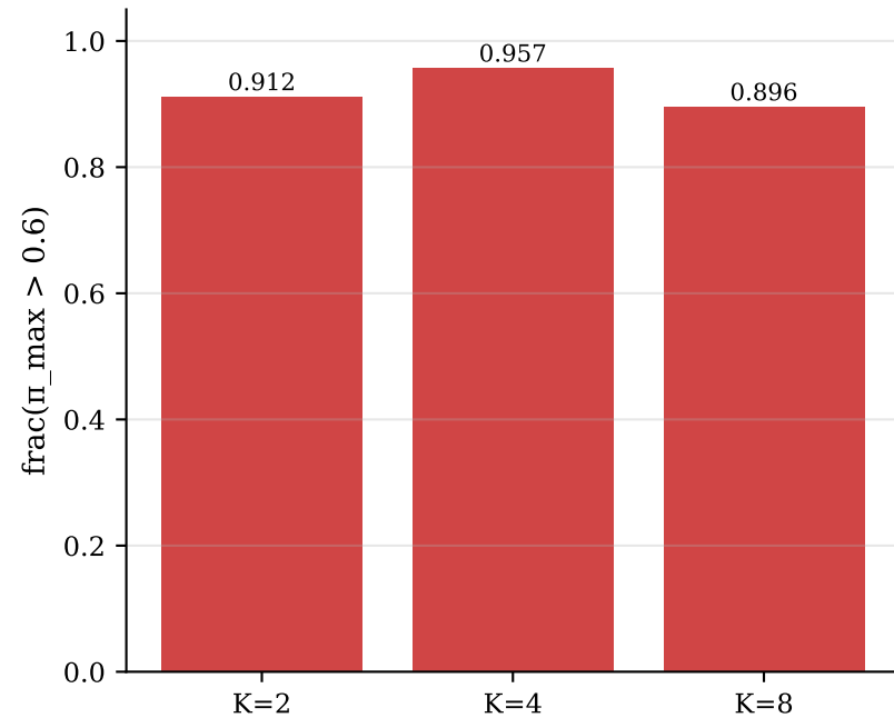
Router saturation (tokens with high-confidence routing)
