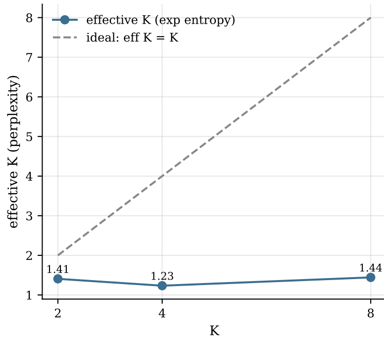
Effective K — capacity utilization
