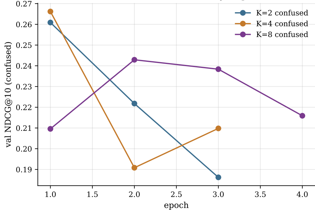
Val NDCG@10 confused — early-stop curve
