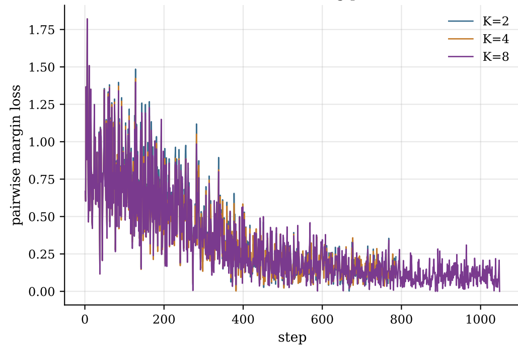
Train loss (all K — overfitting pattern check)
