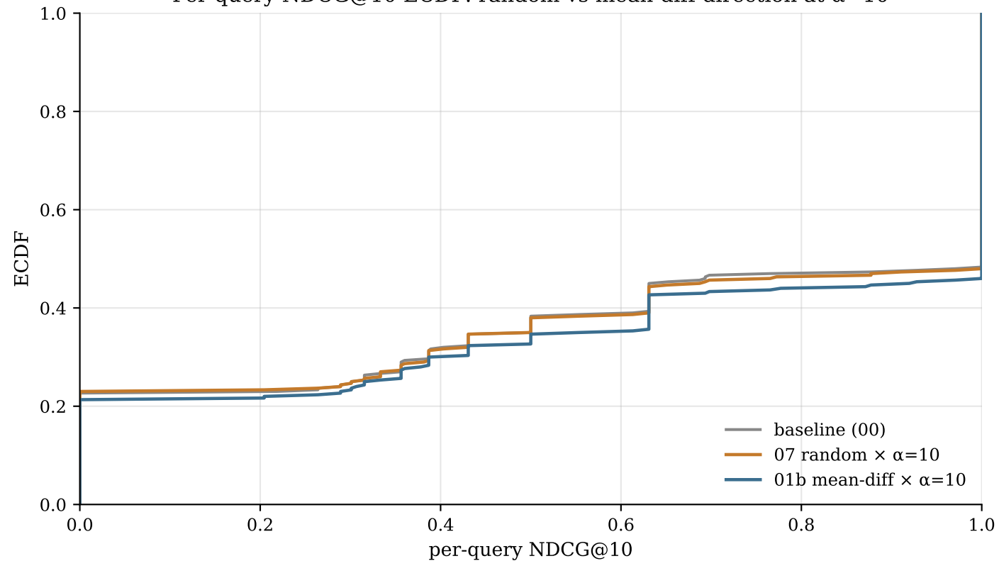
Per-query NDCG@10 ECDF: random vs mean-diff direction at \alpha=10
