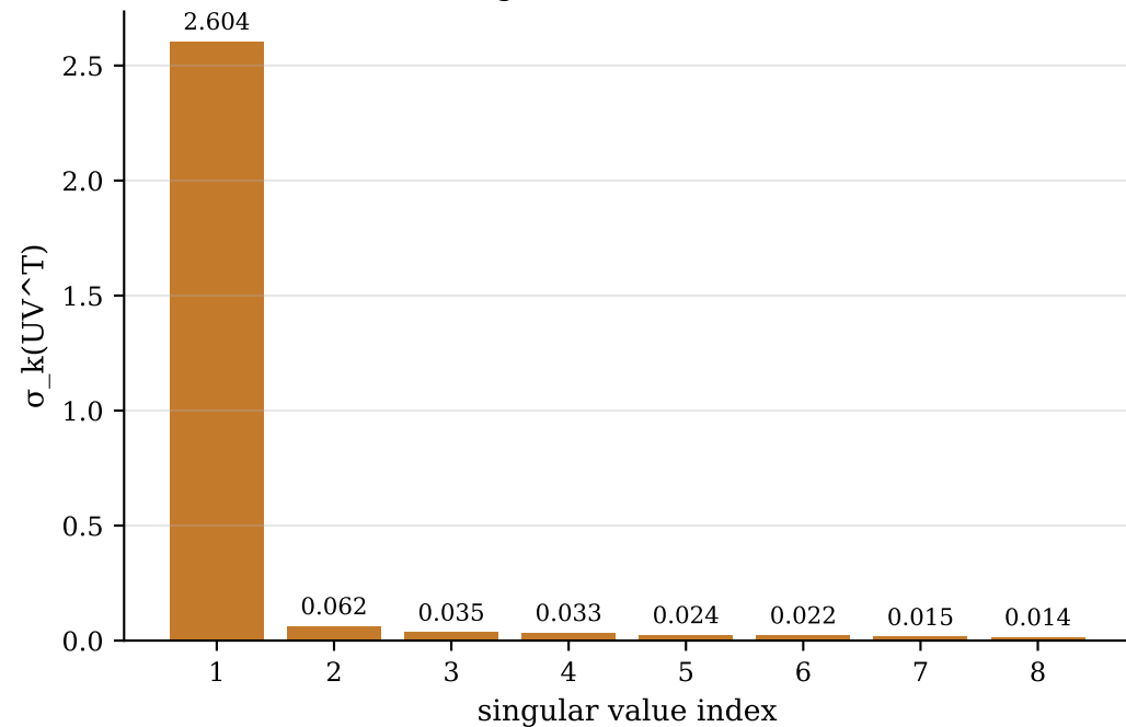
UV T singular values (rank \leq r=8 )
