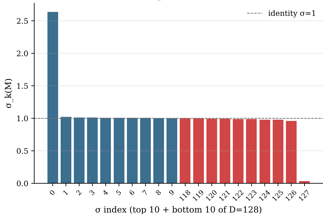
M = I + UV^T spectrum (cond = 81.139)
