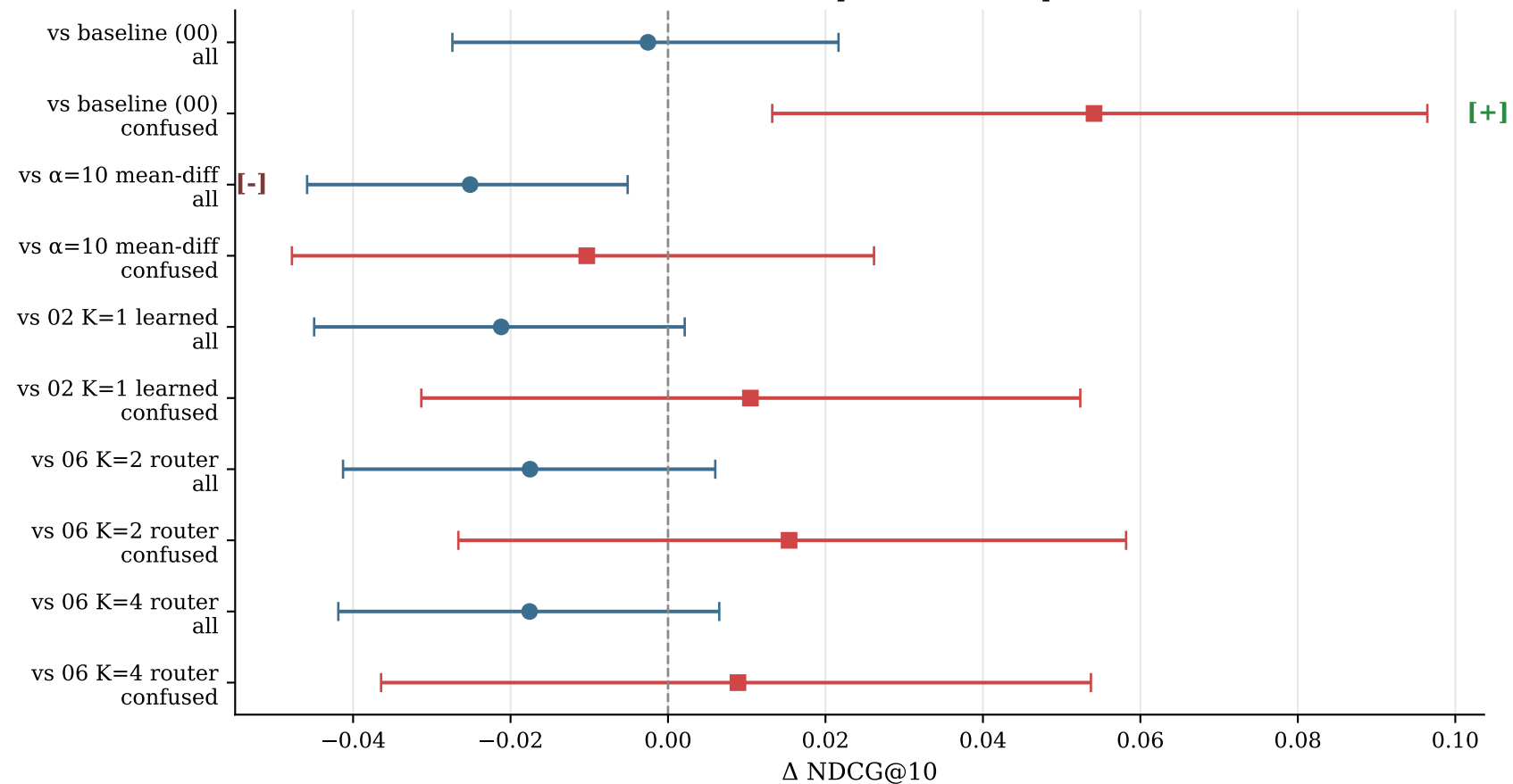
08 bilinear M r=8 — paired bootstrap 95% CI
