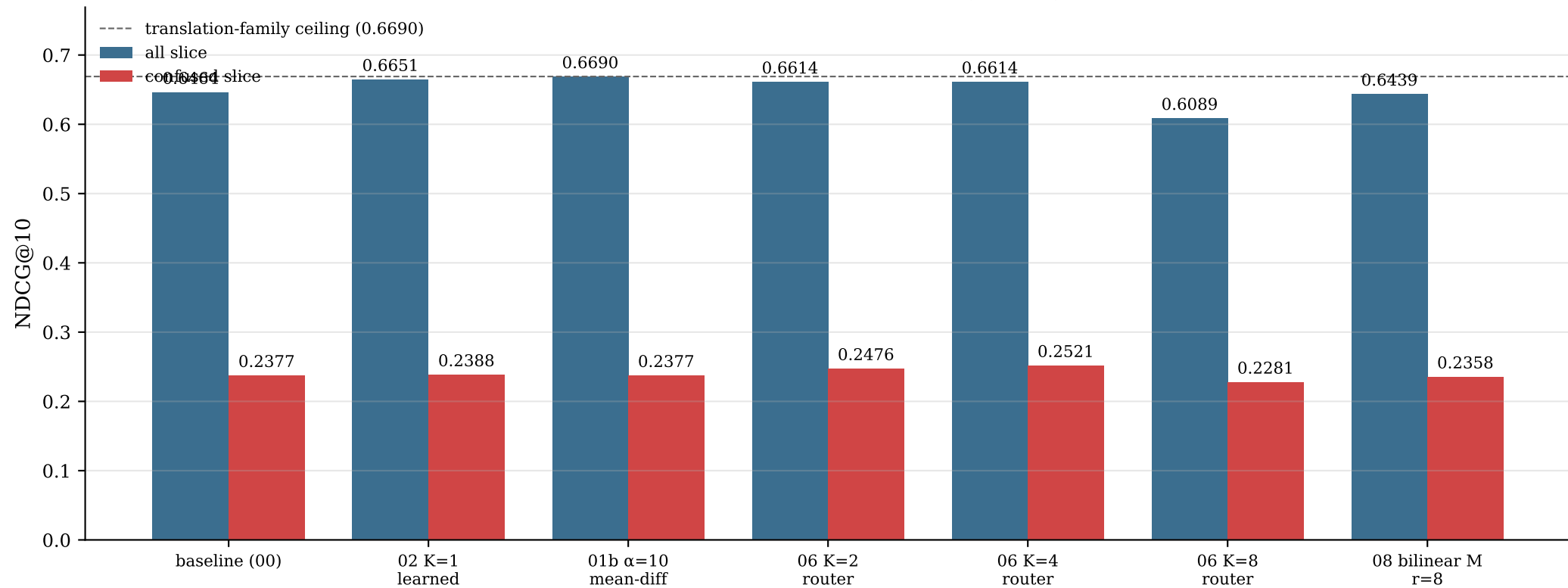
08 bilinear M r=8 — translation-family ceiling test
