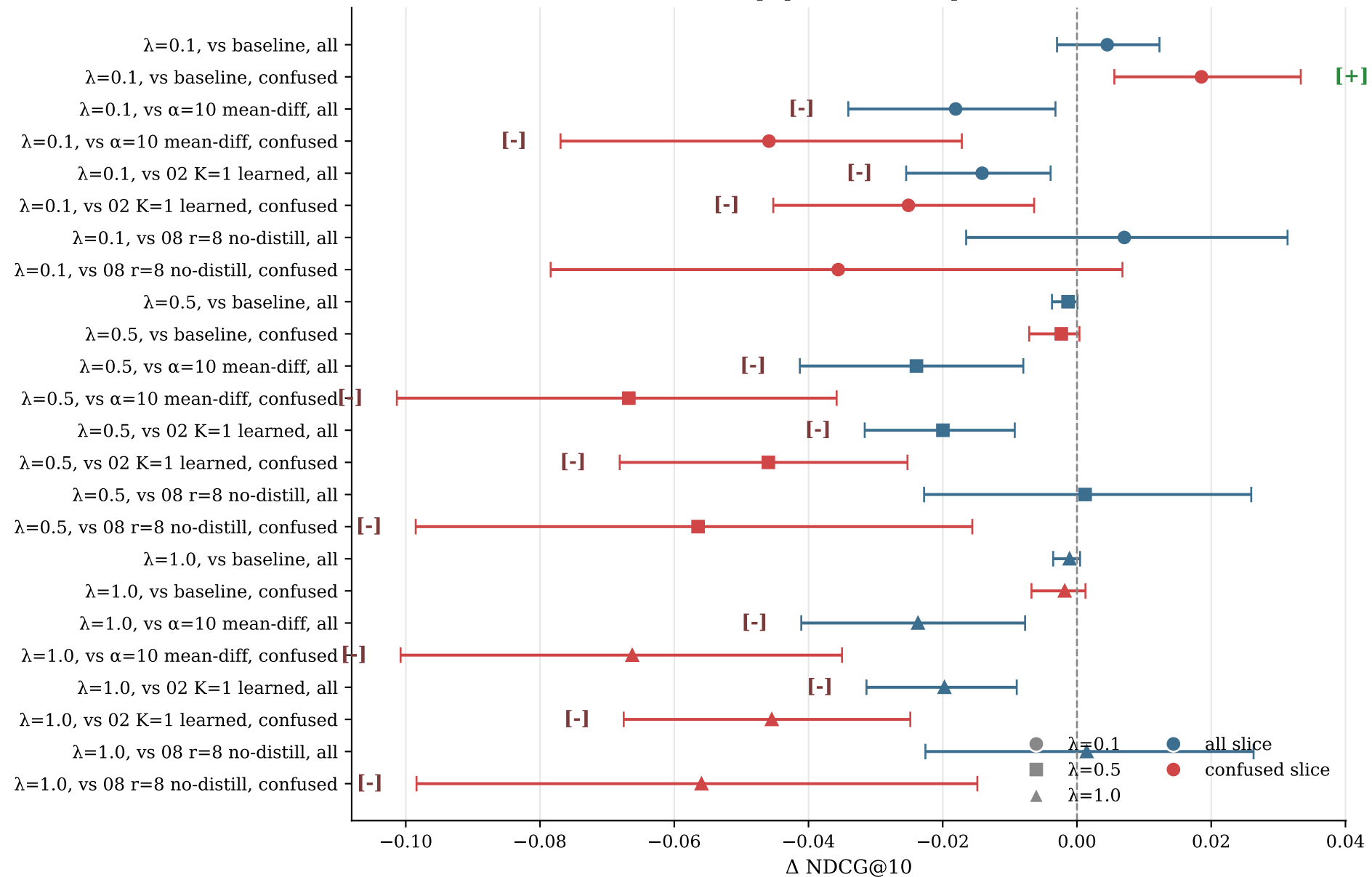
09 \lambda -sweep: paired bootstrap 95% CI
