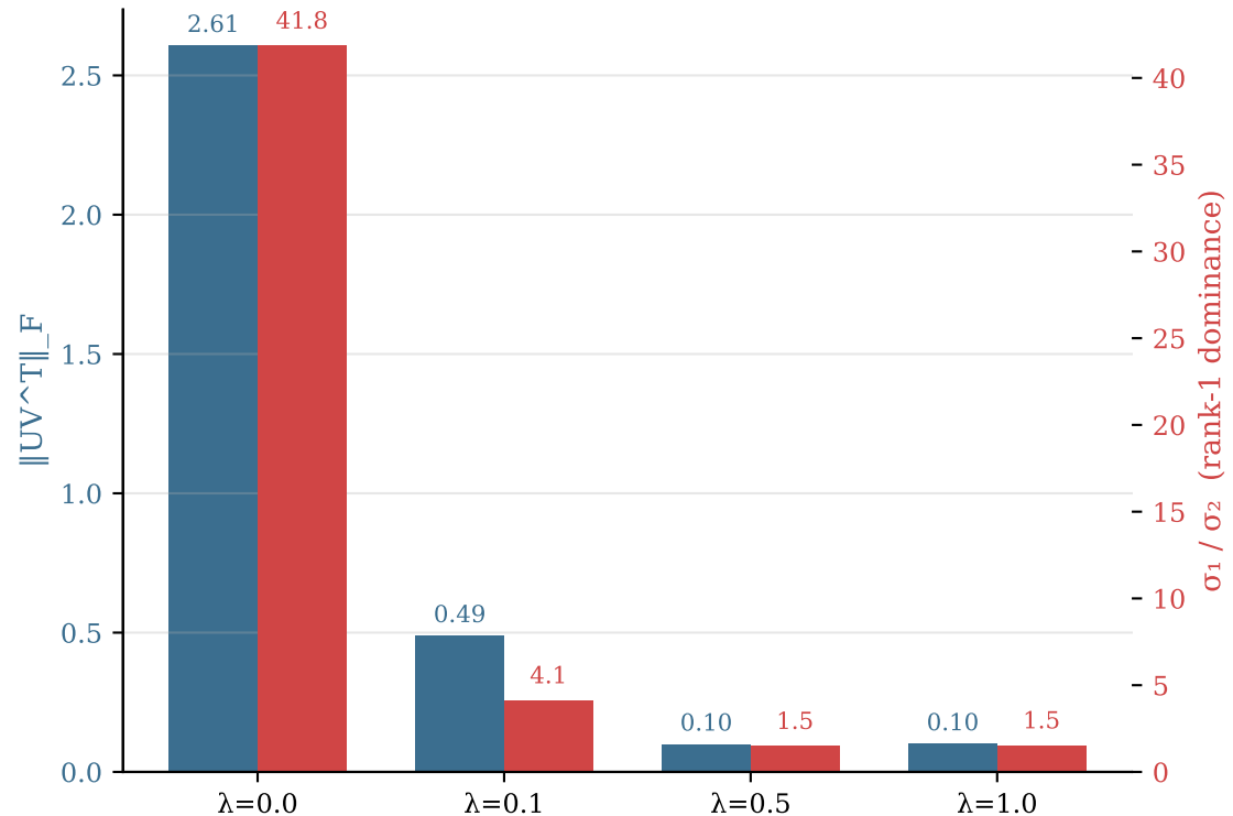
Magnitude vs rank-1 dominance trade-off
