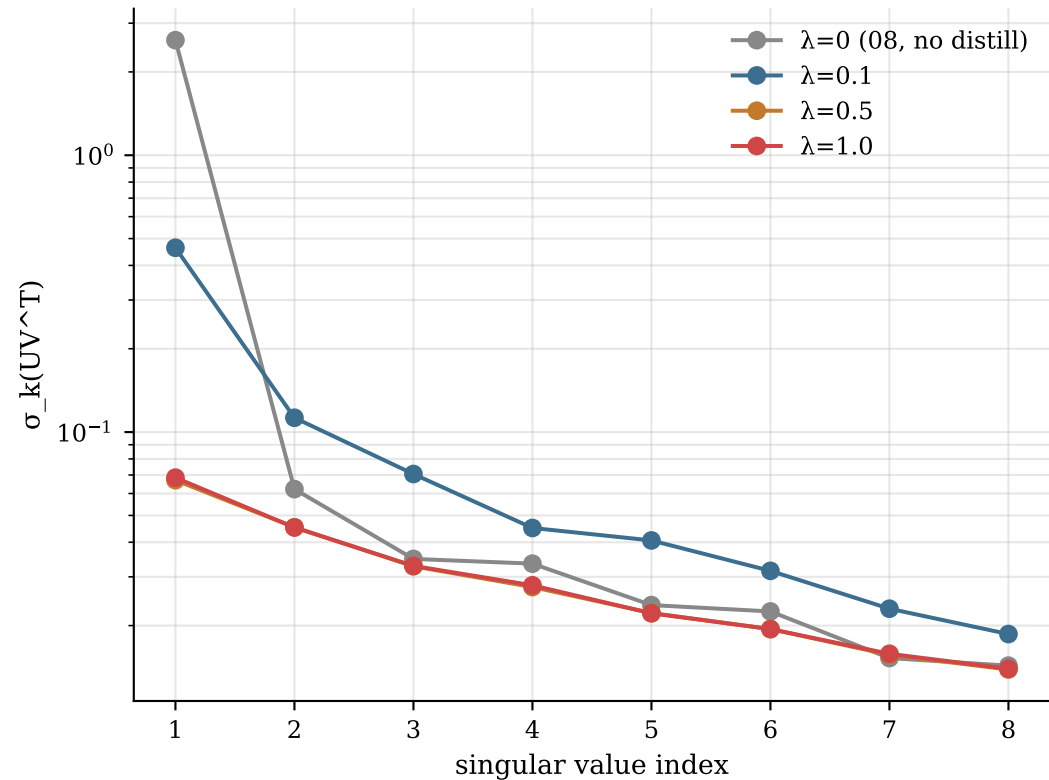
UV T spectrum by \lambda_{\text{distill}} (rank-collapse)
