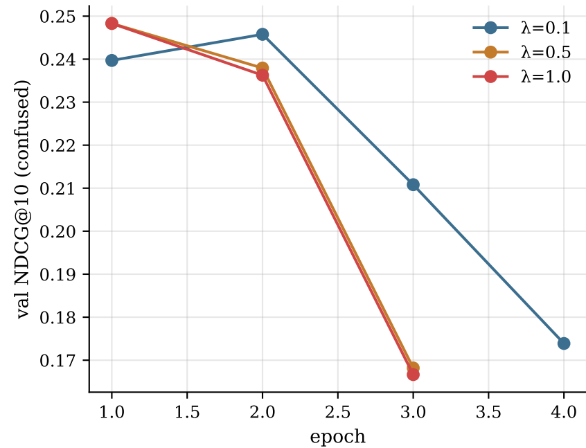
Validation confused-slice
