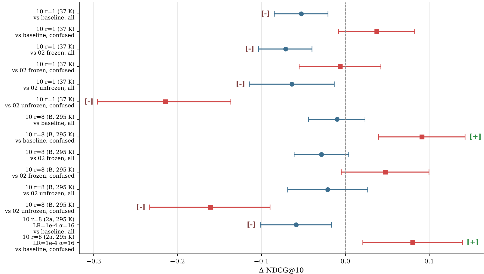
10 LoRA — paired bootstrap 95% CI
