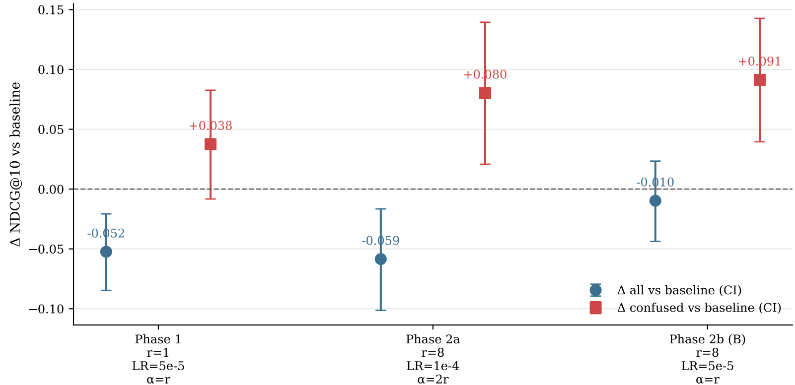
10 LoRA progression: 1 \rightarrow 2a \rightarrow 2b (anchor preservation \square\square )
