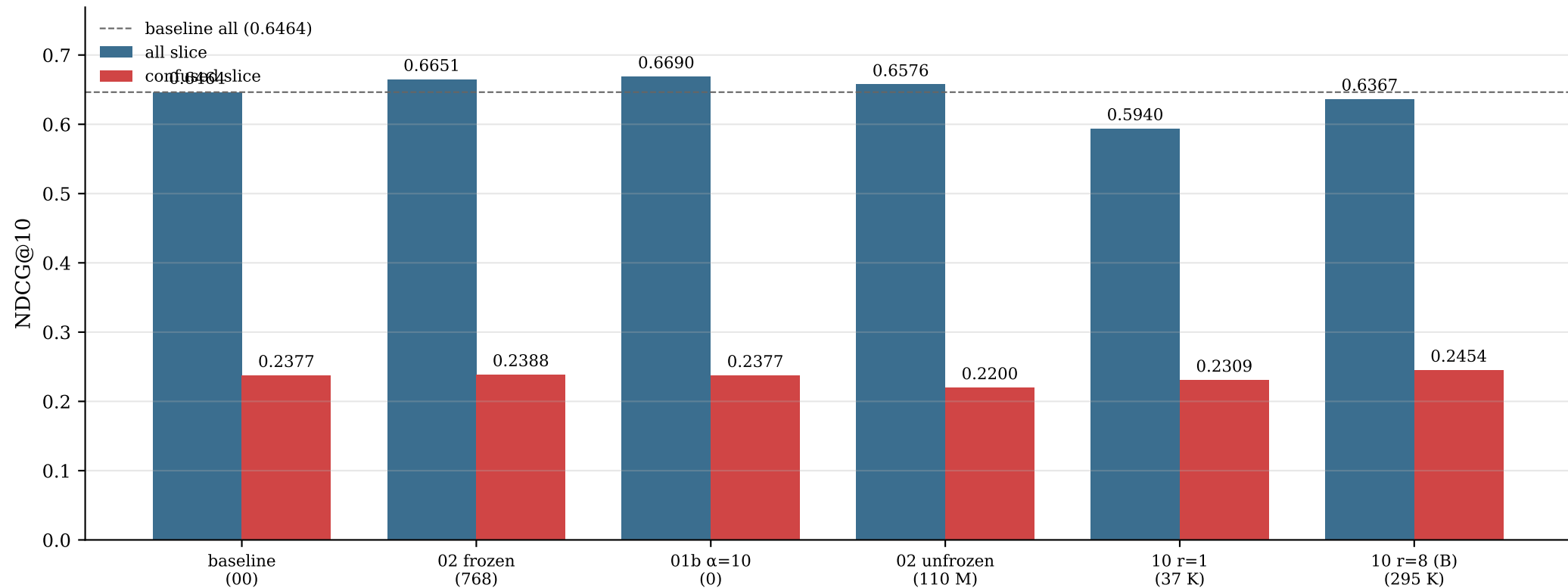
10 LoRA on \Phi — SciFact NDCG@10 vs anchors
