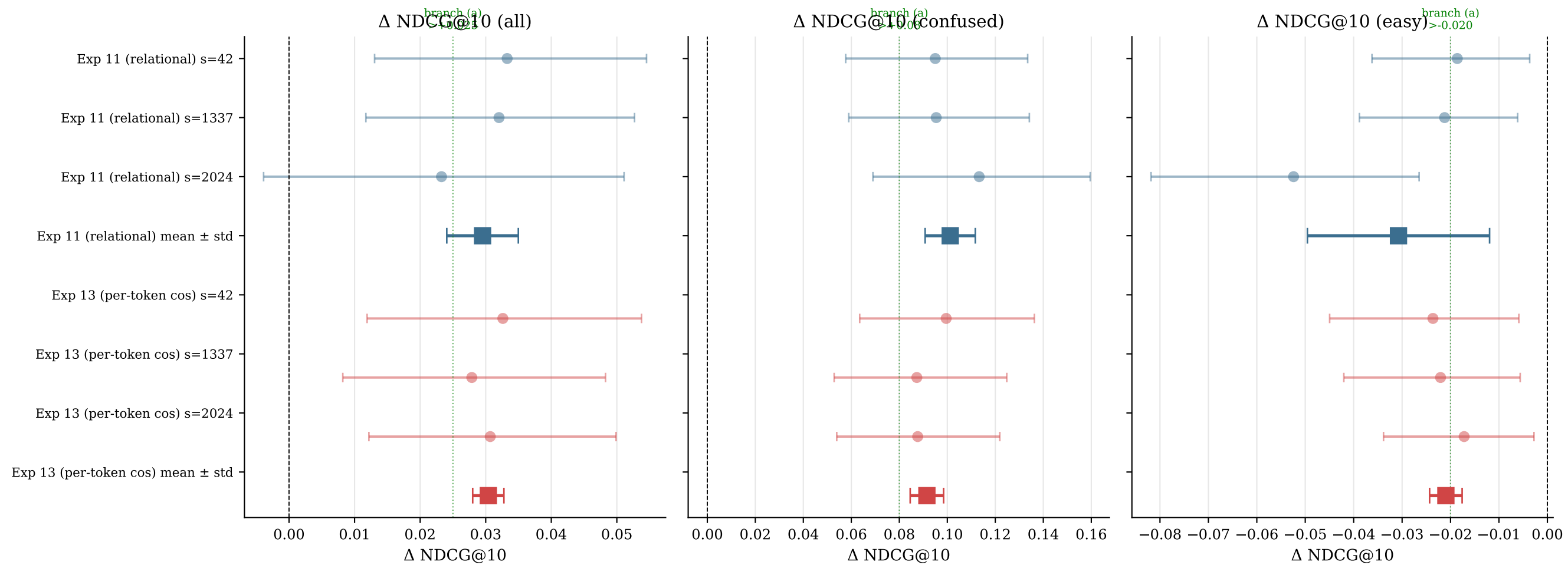
Exp 13 (per-token cosine) vs Exp 11 (Sim Frobenius 2 ) — anchor-side family on SciFact (3 seeds)
