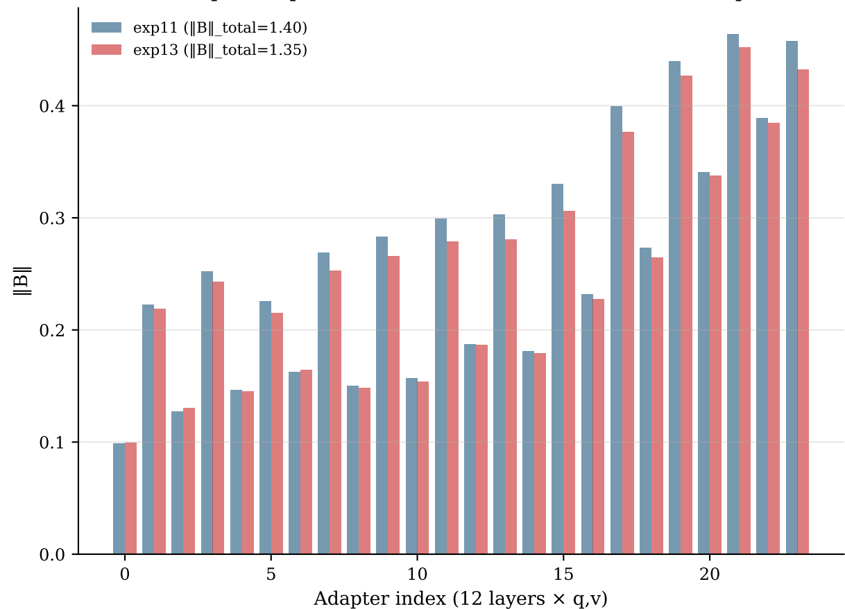
LoRA B norms per adapter (seed 42) — direct measure of anchor preservation
