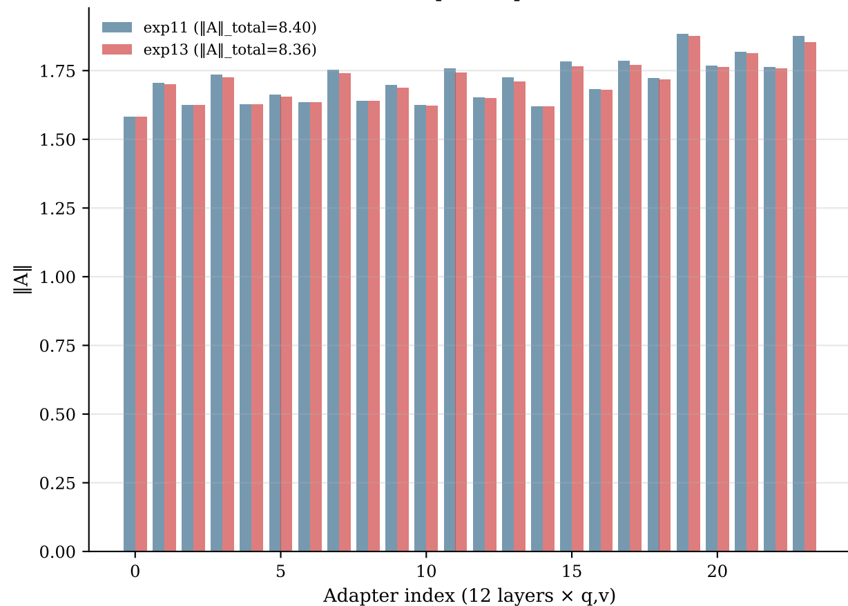
LoRA A norms per adapter (seed 42)
