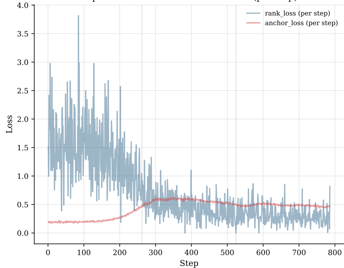
Exp 13 seed 42 — rank + anchor loss (per step)
