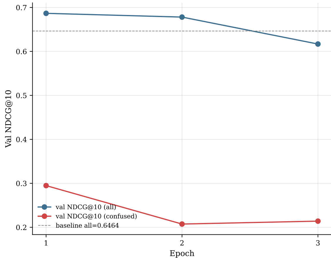
Exp 13 seed 42 — validation NDCG@10
