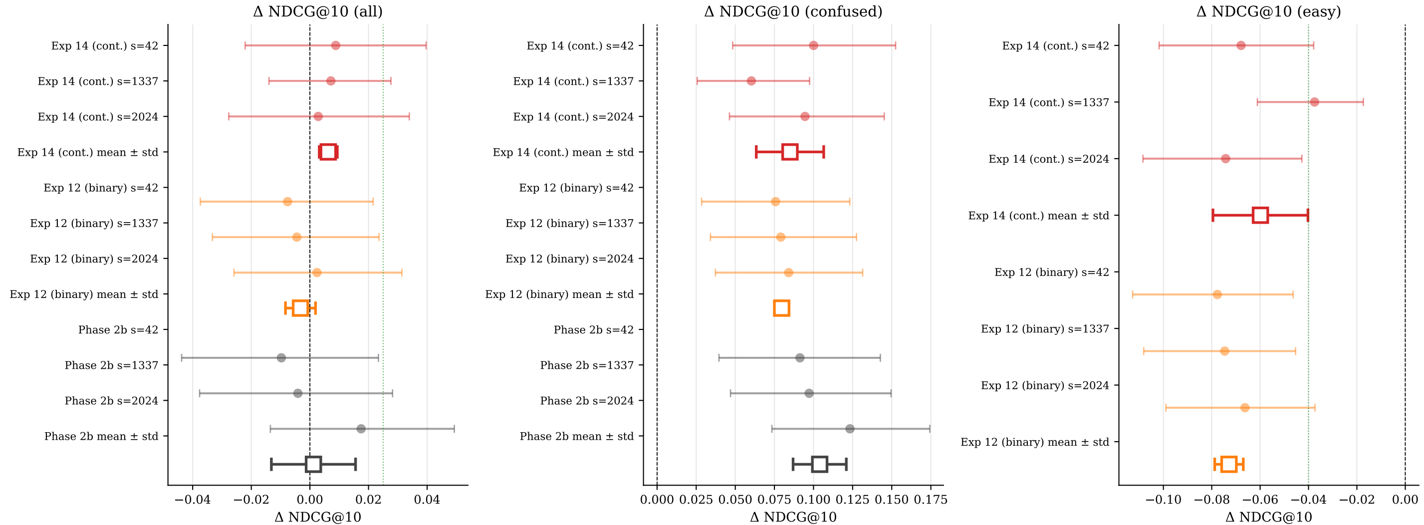
Exp 14 (continuous sigmoid) vs Exp 12 (binary FN cut) vs Phase 2b — SciFact (3 seeds)
