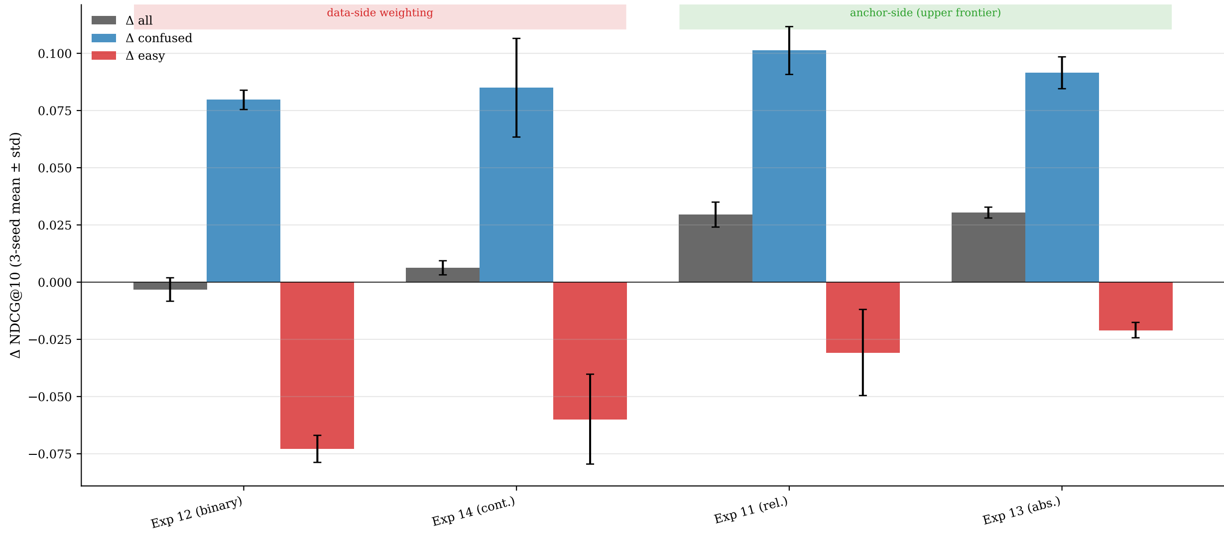
6-lever framework — 3-seed mean \Delta NDCG@10 (SciFact)
