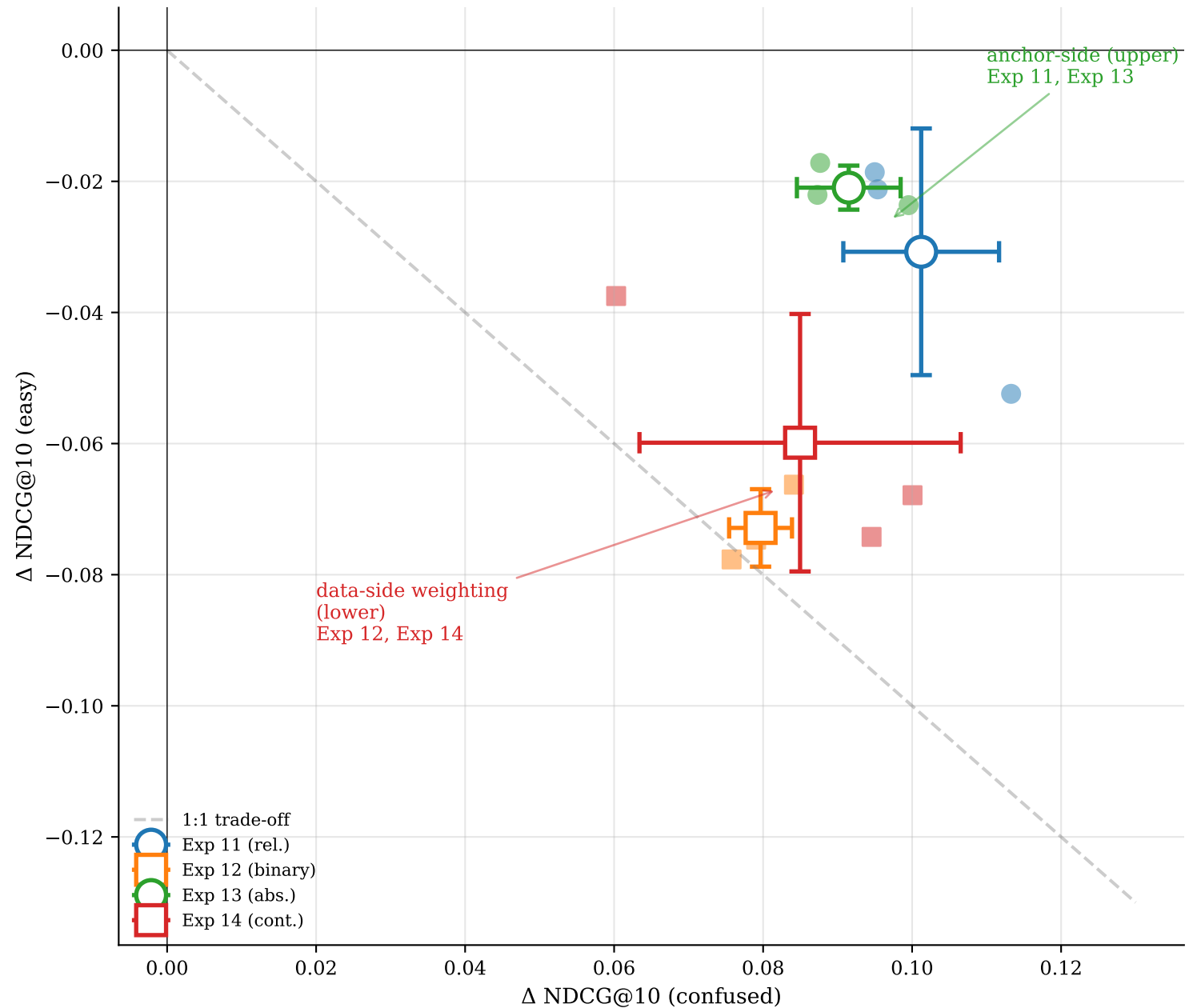
Six-lever trade-off frontier — family-separated structure (SciFact, 3 seeds)
