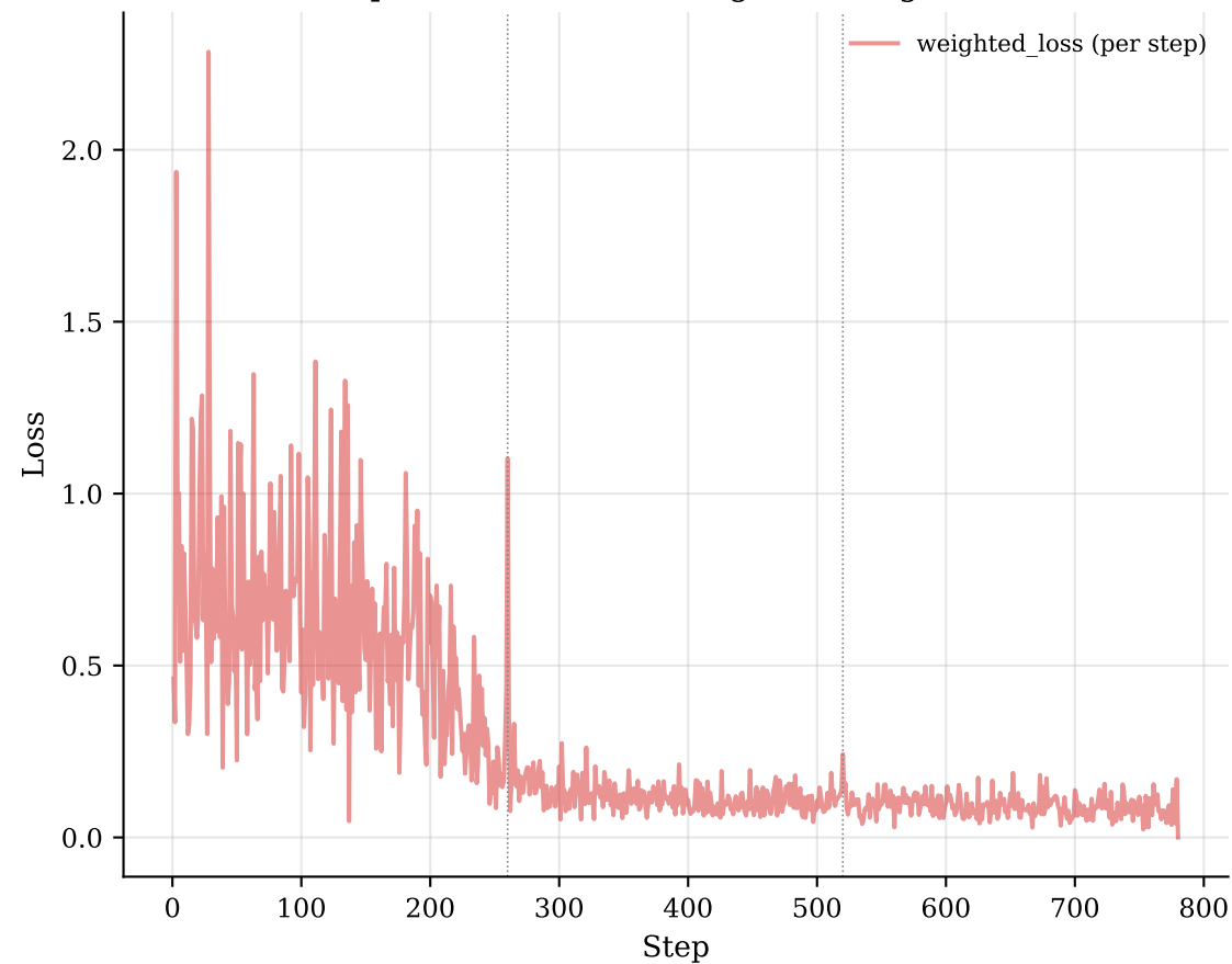
Exp 14 seed 2024 — weighted margin loss
