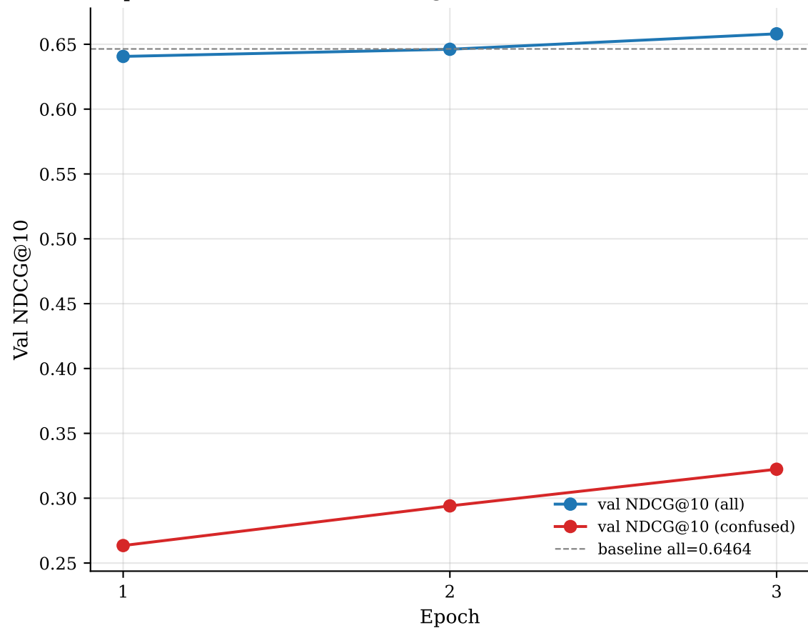
Exp 14 seed 2024 — val NDCG@10 (monotone increase, late best)
