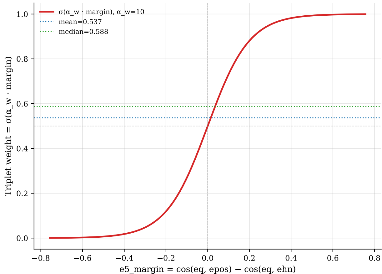
Sigmoid weight vs e5_margin ( \alpha_w=10 )
