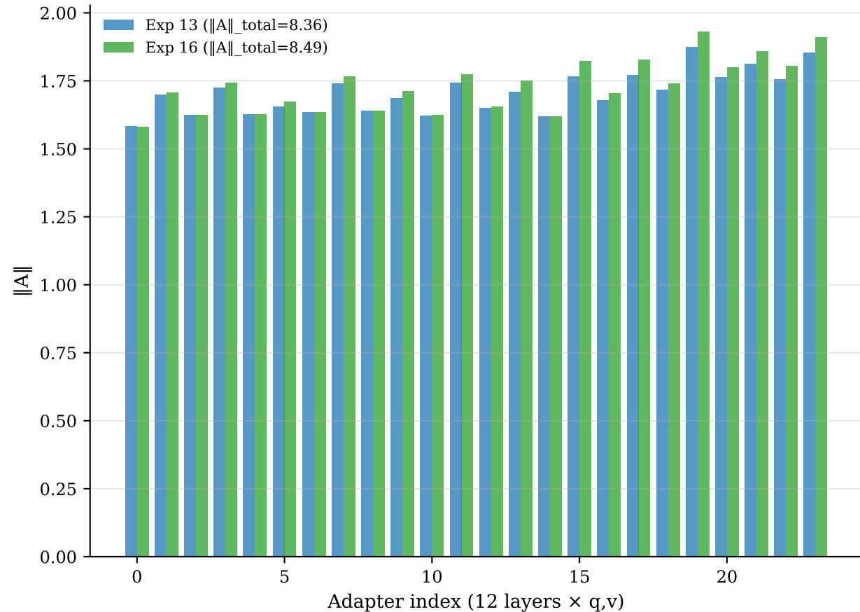
LoRA A norms per adapter (seed 42)
