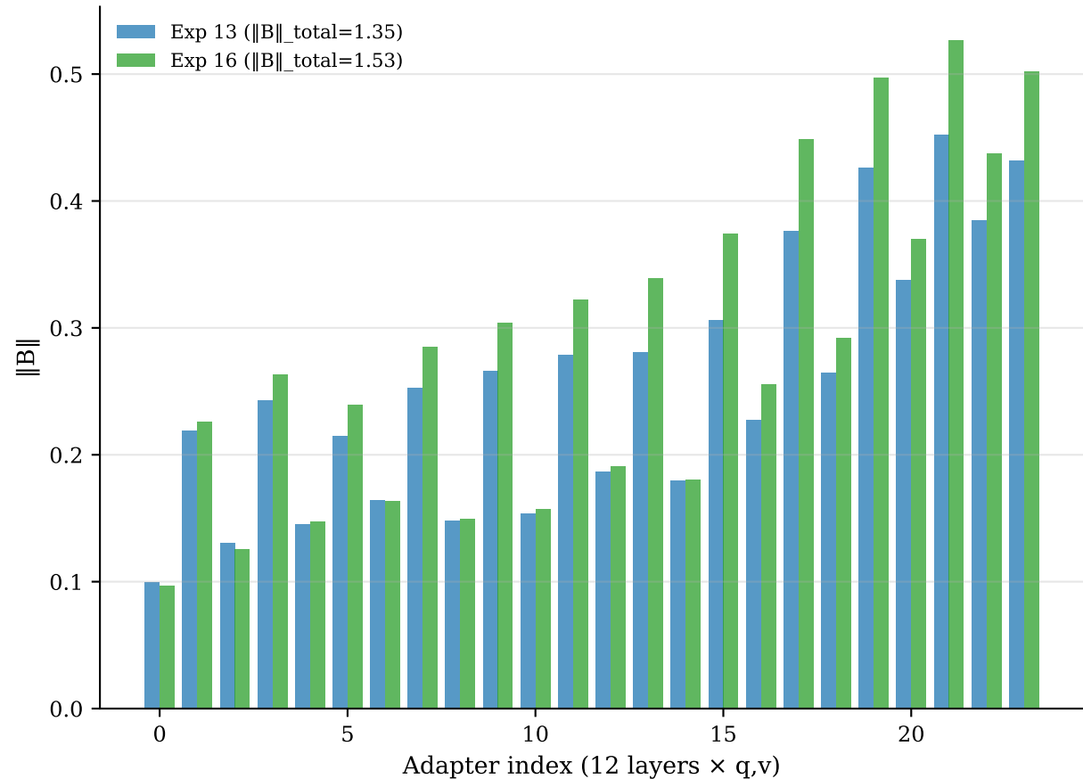
LoRA B norms per adapter (seed 42)
