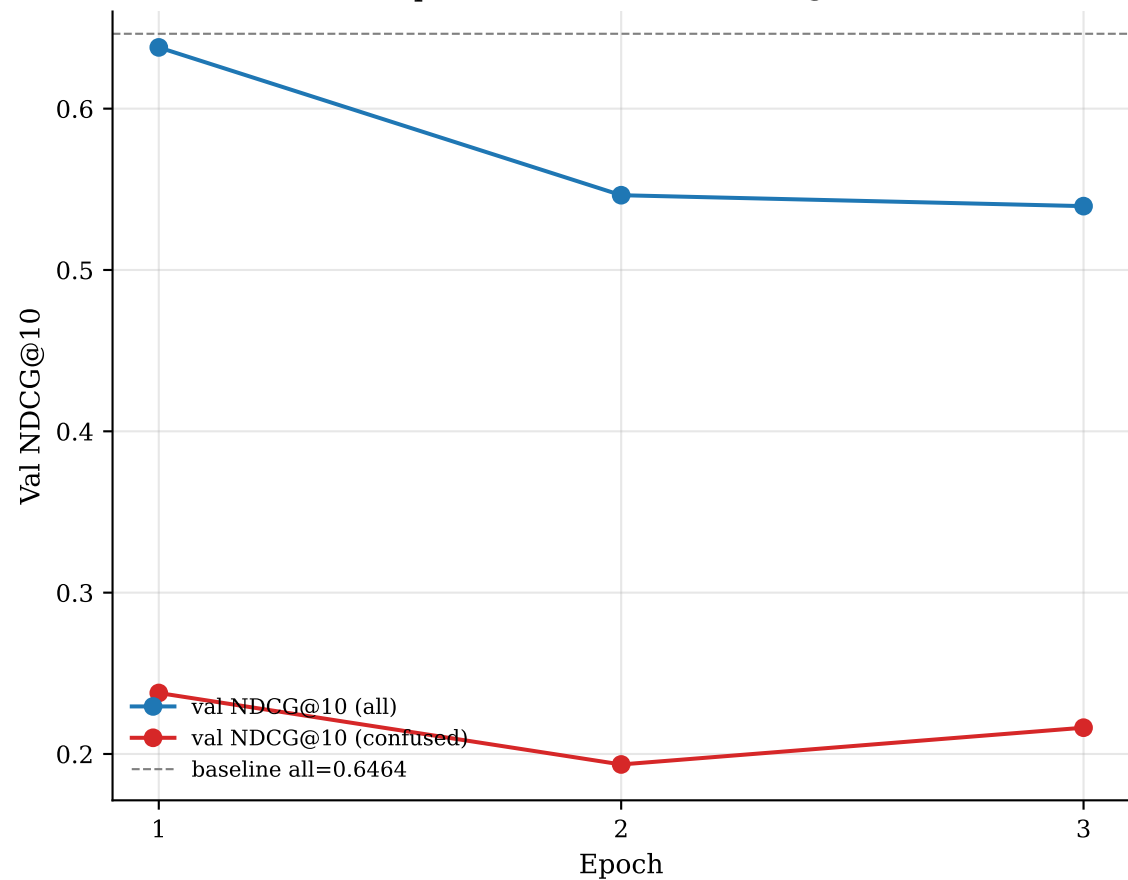
Exp 16 seed 42 — val NDCG@10
