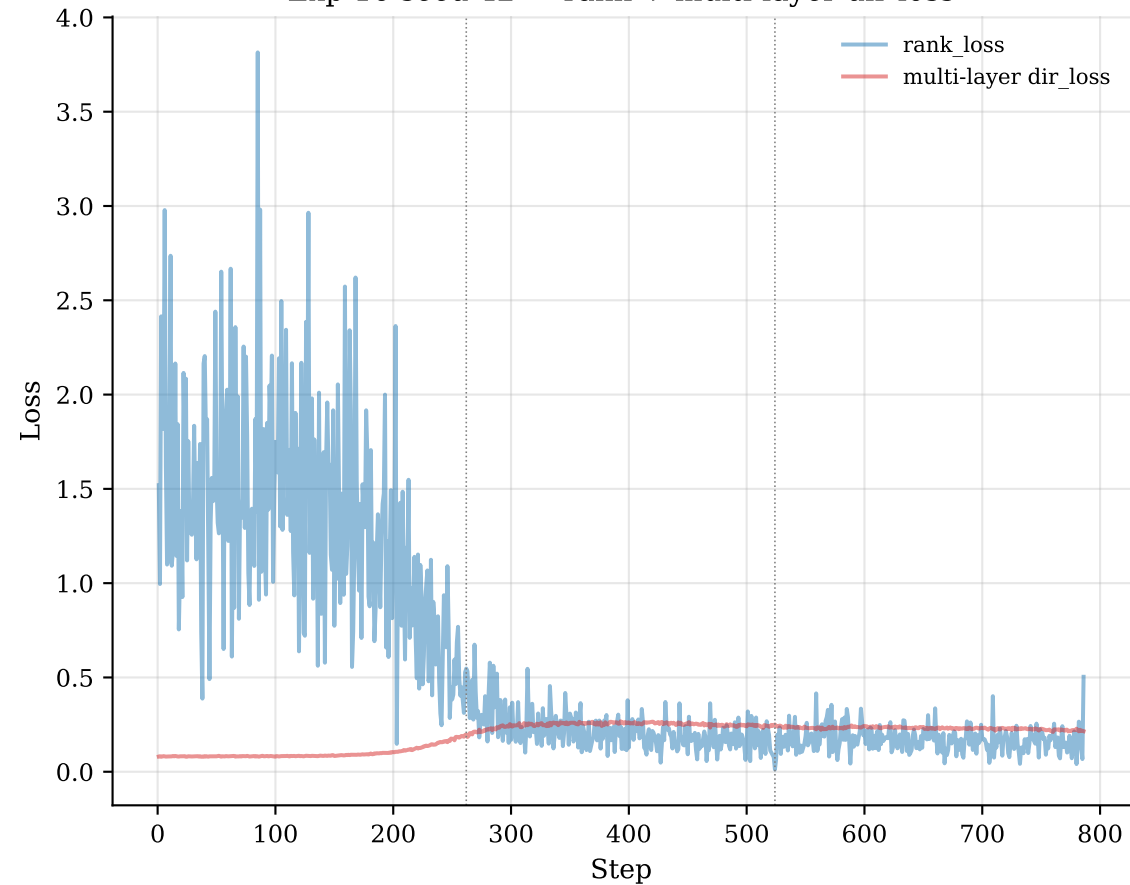
Exp 16 seed 42 — rank + multi-layer dir loss
