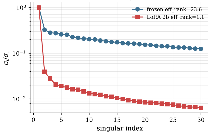
fiqa — token singular spectrum
