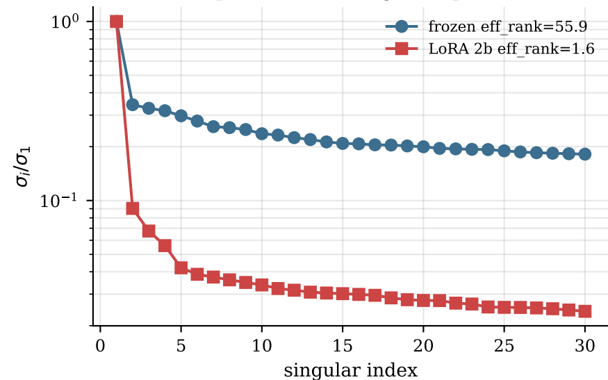
nfcopus — token singular spectrum
