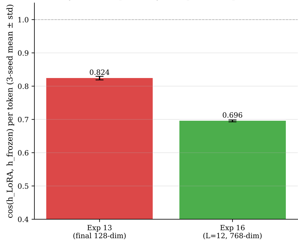
Final-layer anchor proximity — Exp 13 vs Exp 16 (at L=12)
