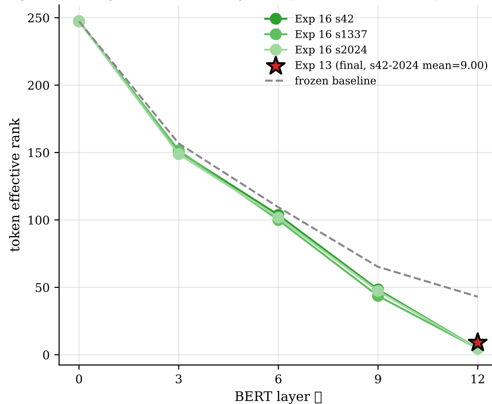
Per-layer token diversity — Exp 16 vs frozen + Exp 13 ref
