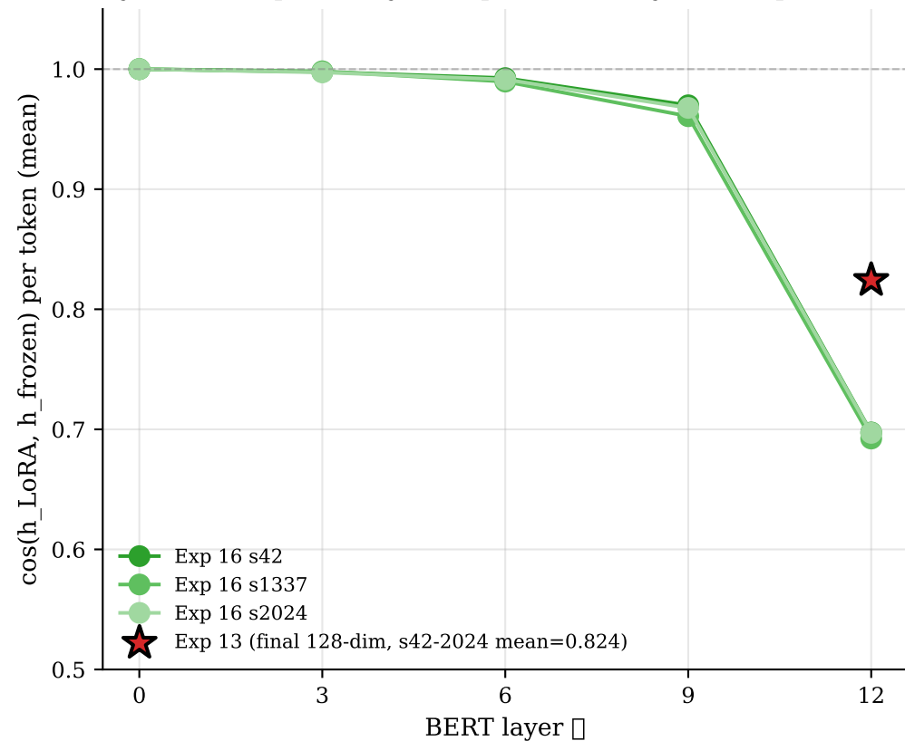
Per-layer anchor proximity — Exp 16 multi-layer vs Exp 13 final-only
