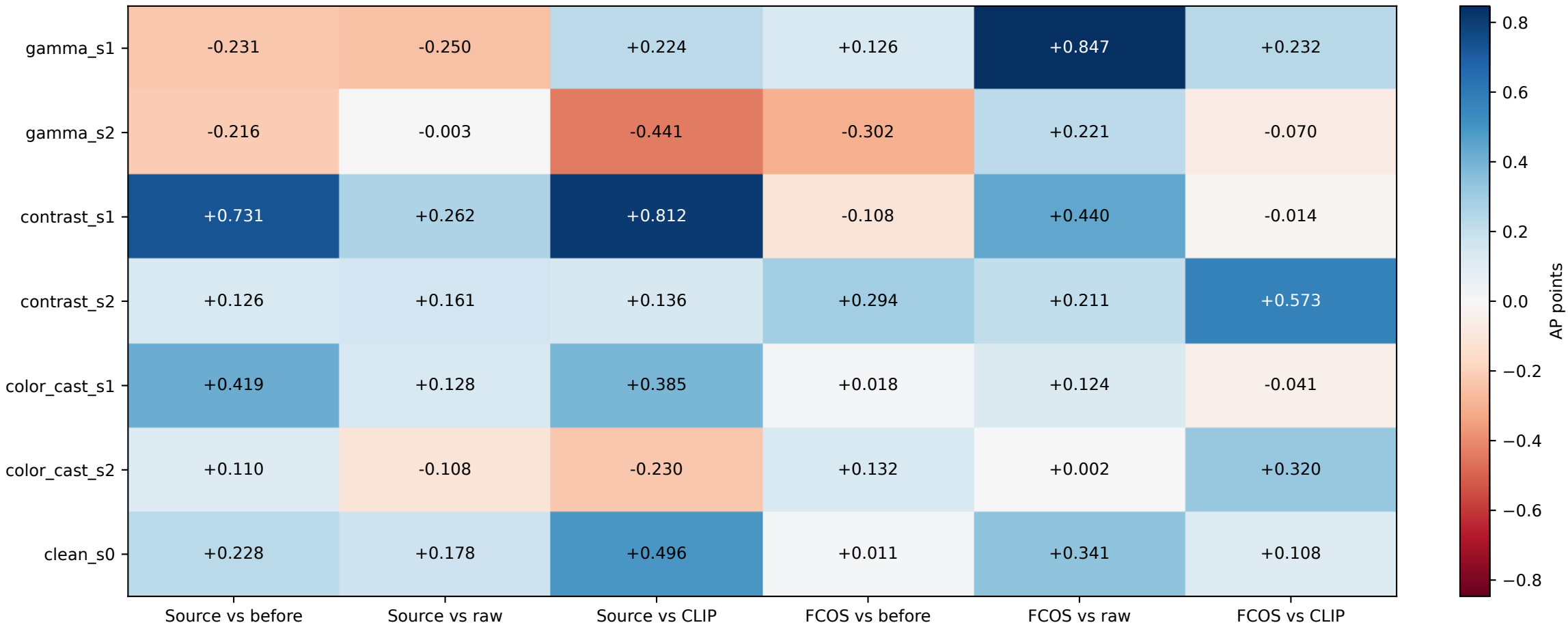
T007 disjoint subset: hybrid AP change after 3 steps
