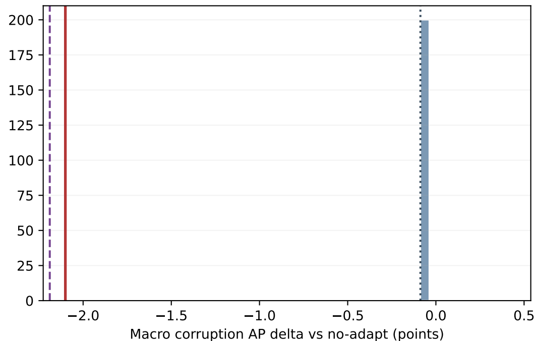
SSD300-VGG16: half-dose -2.1006 AP
