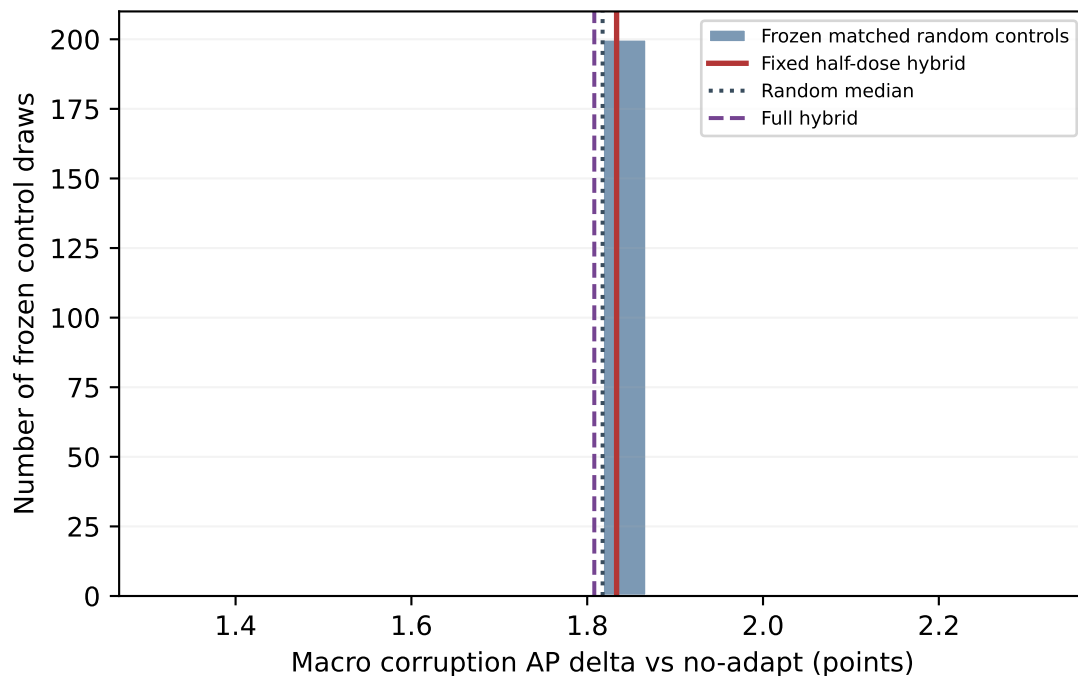
FCOS: half-dose +1.8334 AP
