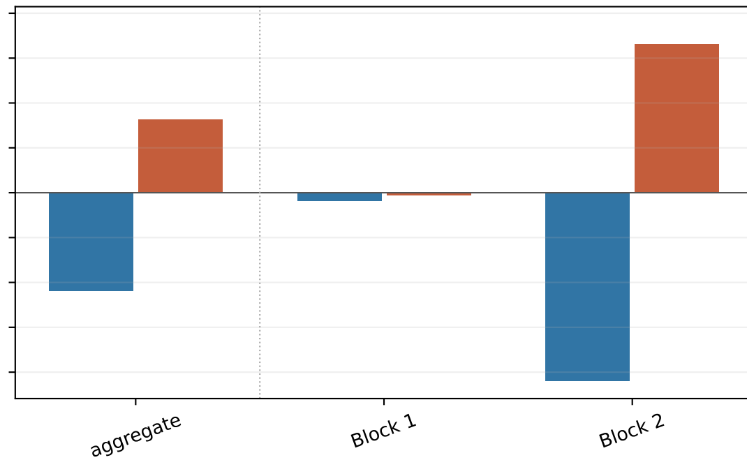
SSD300-VGG16
