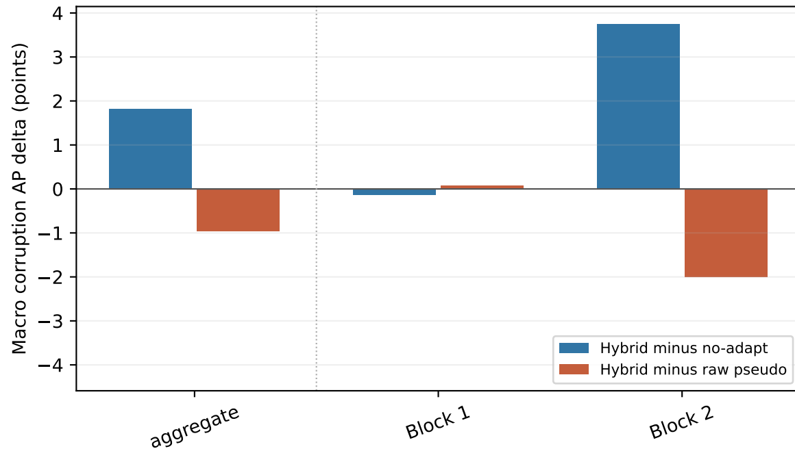
FCOS
