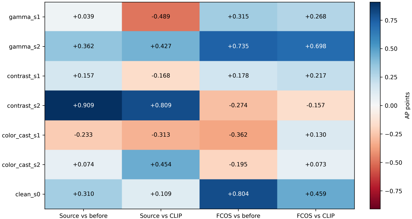
T006: pseudo-confidence AP change after 3 steps
