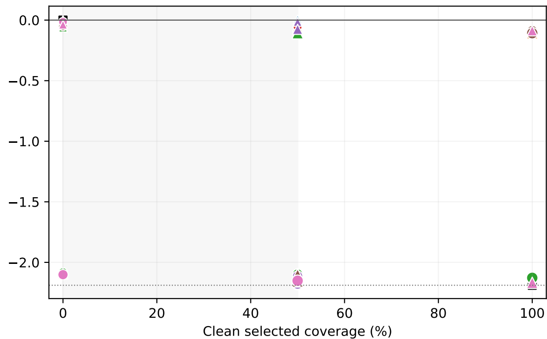
SSD300-VGG16
