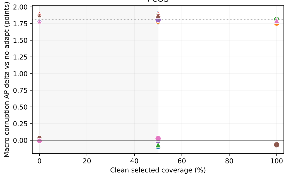
FCOS
