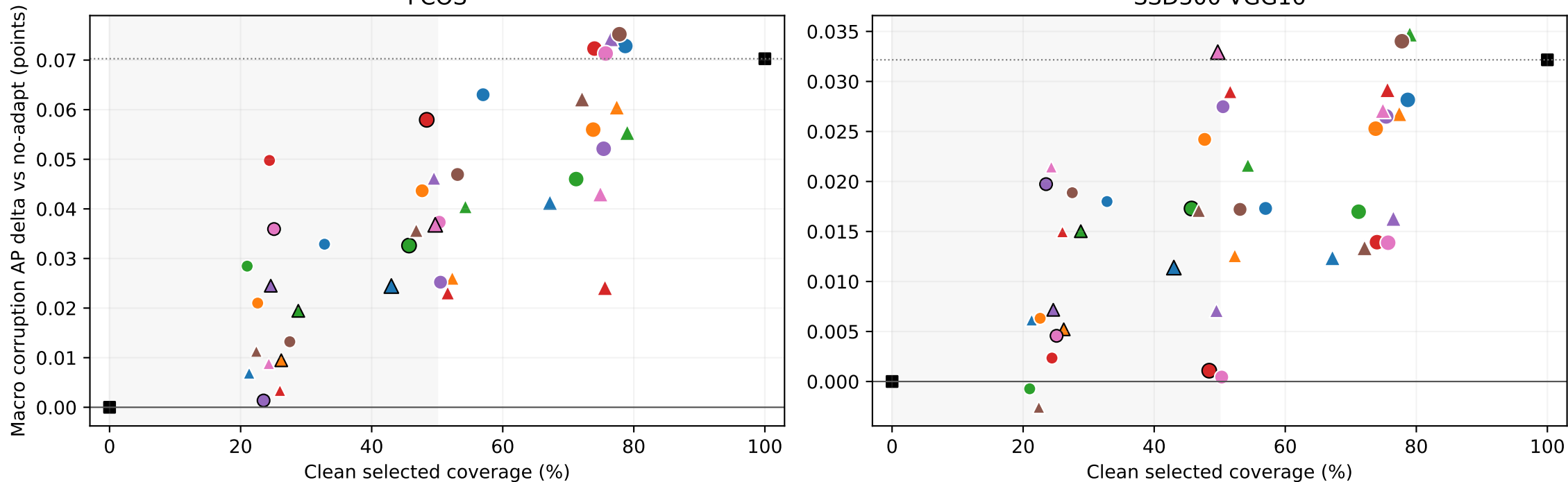
FCOS
