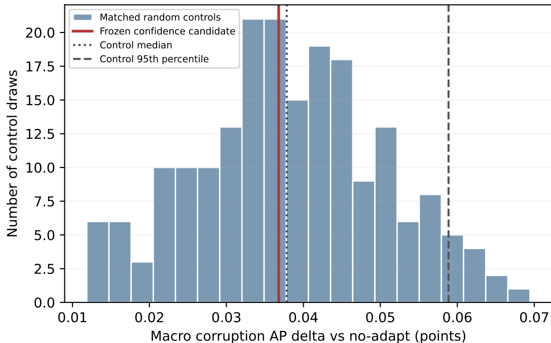
FCOS: percentile 47.0%, tail 0.5323
