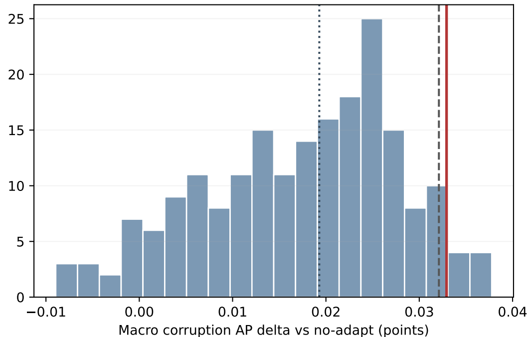
SSD300-VGG16: percentile 96.0%, tail 0.0448
