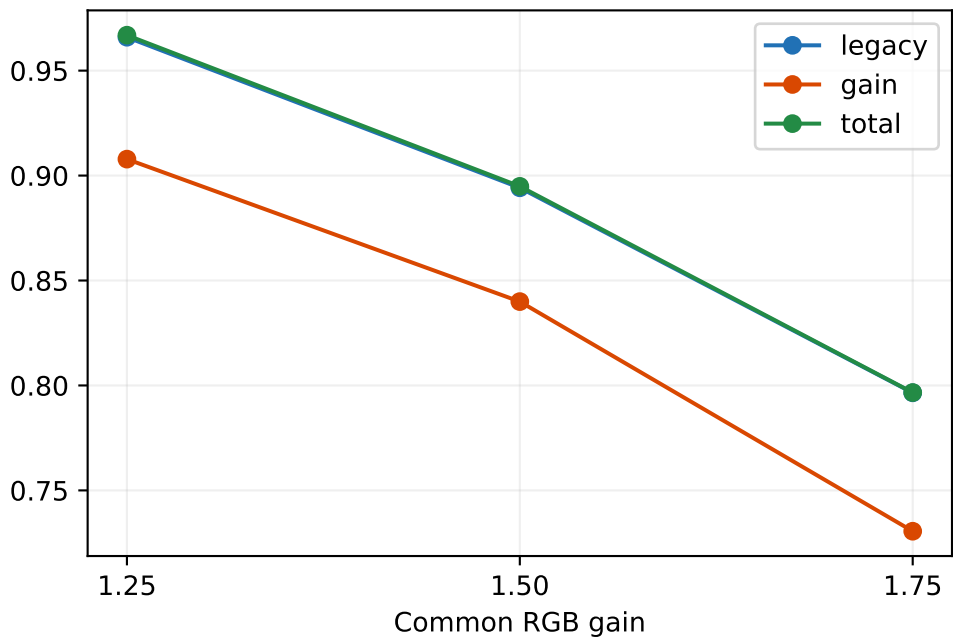
Positive-dot fraction
