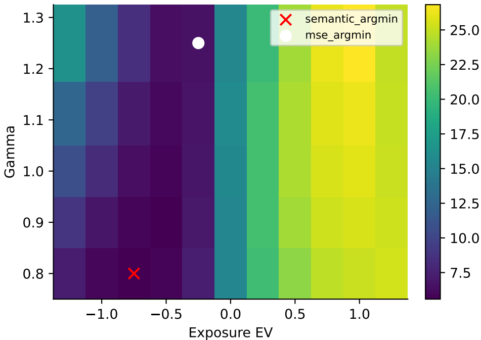
Frozen semantic loss
