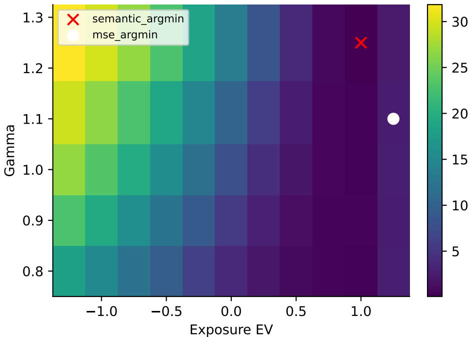
Frozen semantic loss
