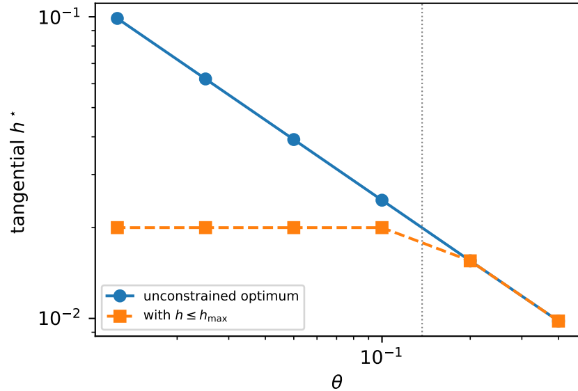
Corollary 7.2: span cap (dotted line: predicted \theta_{c,2} )
