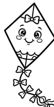
KITE
