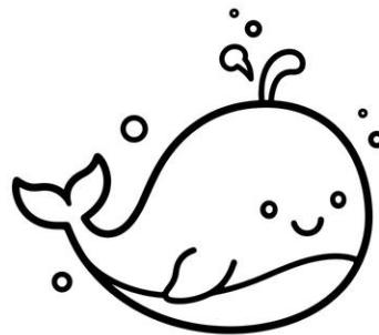
WHALE
